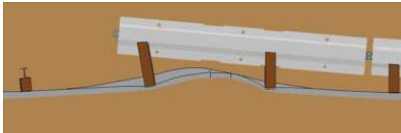
Figure C-3. Localized Kinking Between Oversize Blockouts
