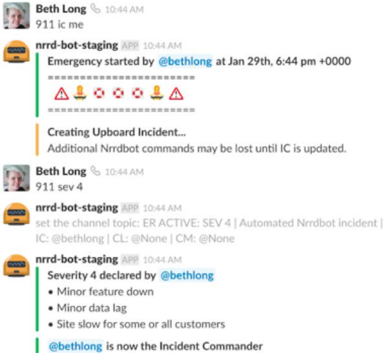
Example incident declared in Slack
