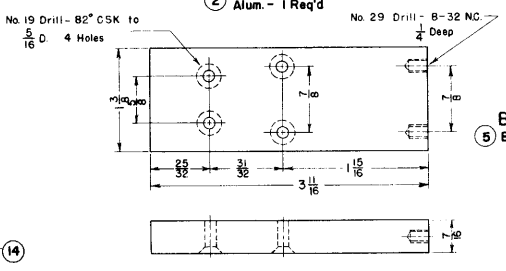
BASE Alum. - 1 Req'd
