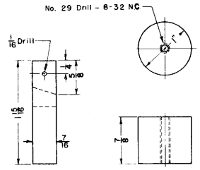
COUNTERBALANCE Brass - 1 Req'd
