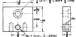
END POST Alum. - 1 Req'd
