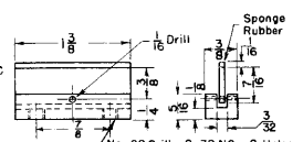
BEAM KNIFE EDGE (swivel) Brass - (2 pieces) 1 unit Req'd.
