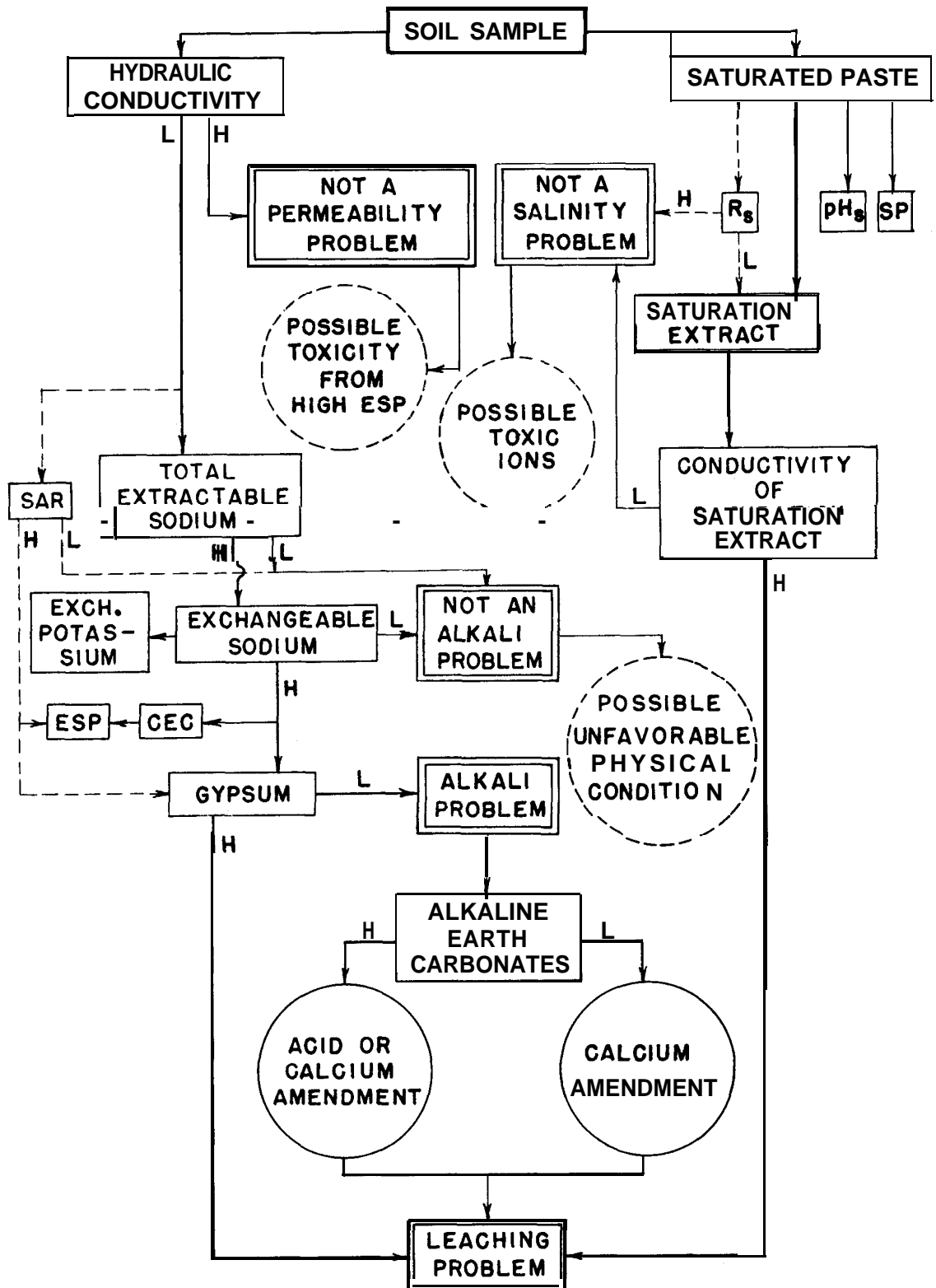
FIGURE II.—Sequence of determinations for the diagnosis and treatment of saline and alkali soils: H , High; L , low; R s , electrical resistance of soil paste; SAR , sodium-adsorption-ratio; ESP , exchangeable-sodium-percentage; CEC , cation-exchange-capacity.
