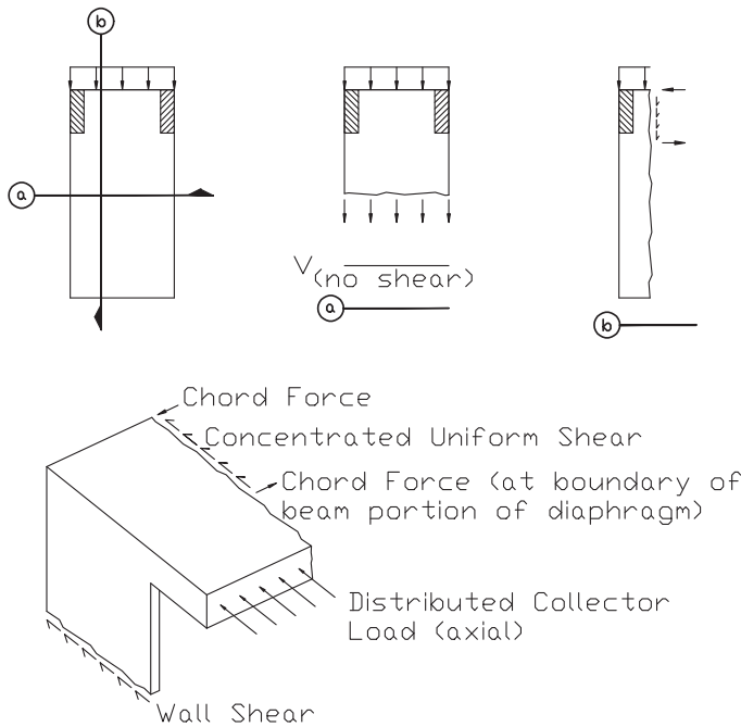
(above) Figure 4: Distributed collector diaphragm
