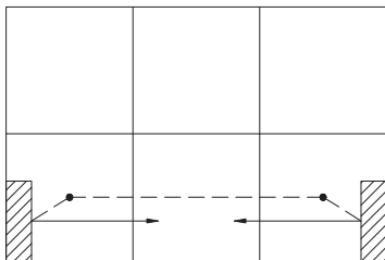
(above) Figure 6: Discretized strut-and-tie diaphragm
