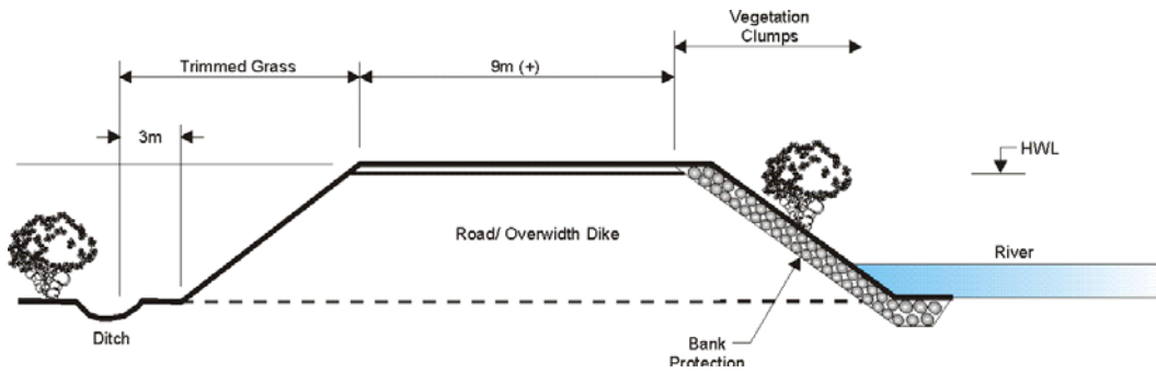
Figure 3 - Overwidth Dike
