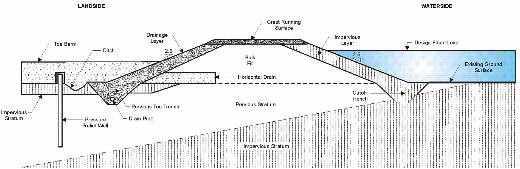
Figure 6 - Potential Seepage Control Options for Design (Not All Required)
