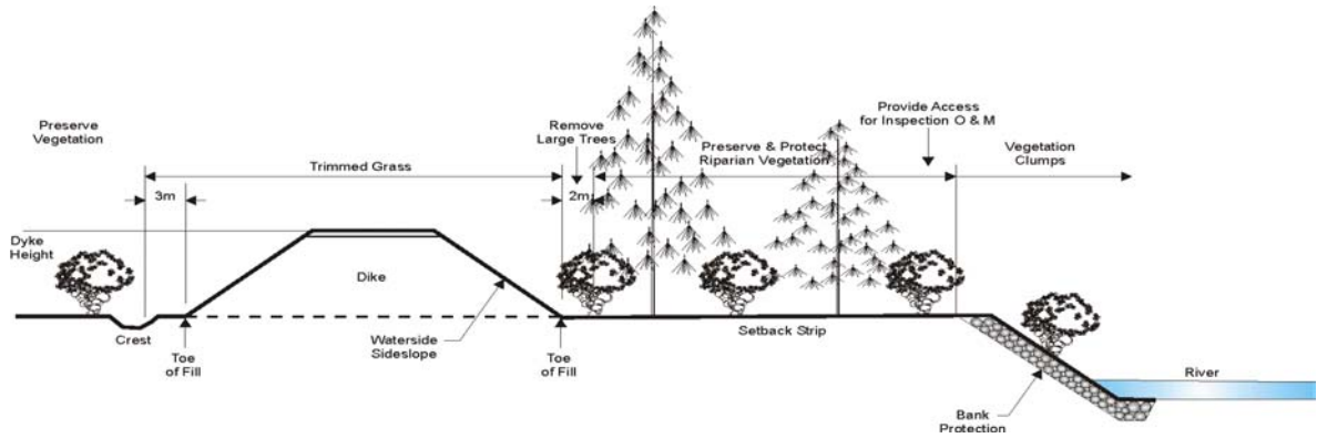
Figure 1 - Setback Dike
