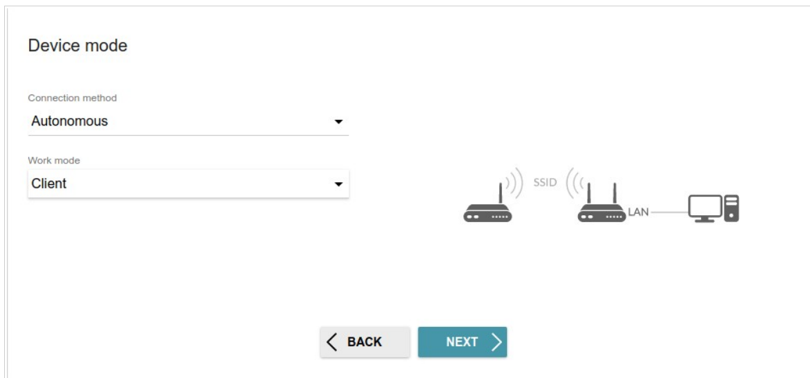
Figure 41. Selecting an operation mode. The Client mode.
