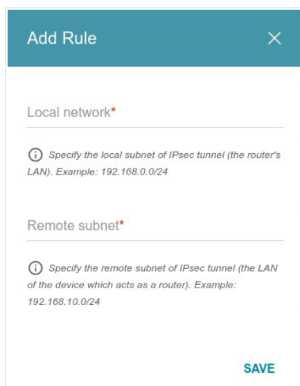
Figure 159. The page for adding an IPsec tunnel. The window for adding a tunneled network.
