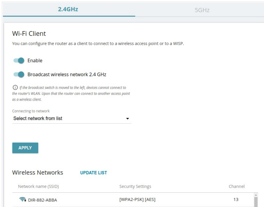
Figure 138. The page for configuring the client mode.
