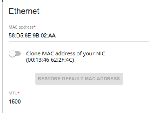
Figure 79. The page for creating a new PPPoE IPv6 connection. The Ethernet section.
