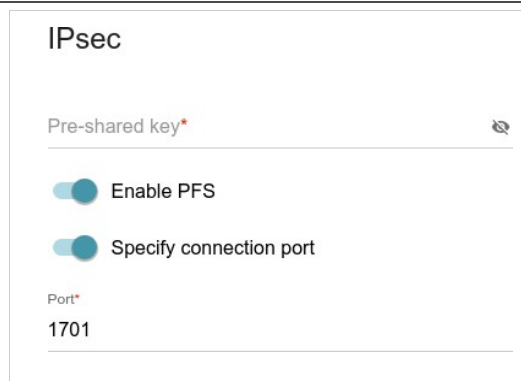
Figure 77. The page for creating a new L2TP over IPsec connection. The IPsec section.
