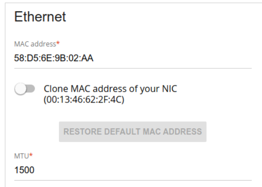
Figure 65. The page for creating a new Static IPv4 connection. The Ethernet section.
