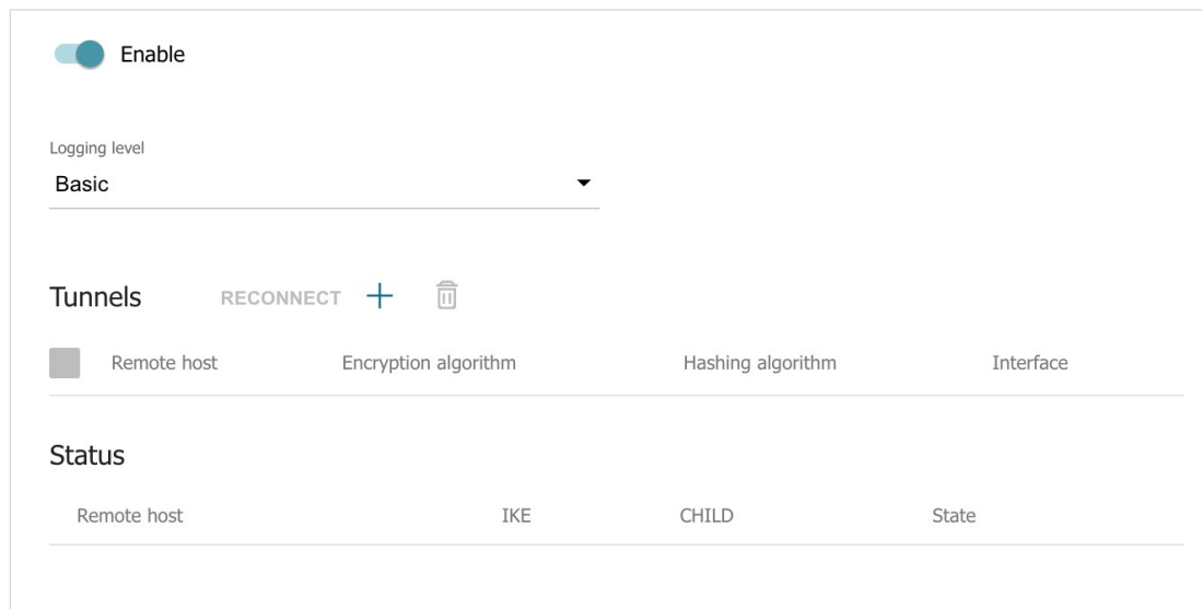
Figure 156. The Functions / Advanced / IPsec page.
