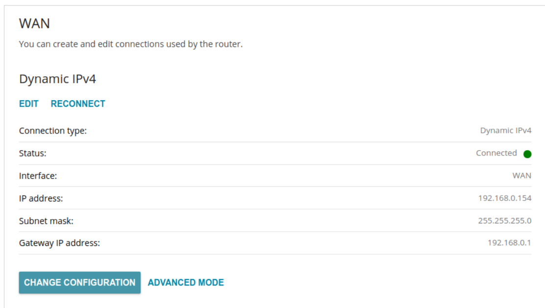
Figure 62. The Settings / Internet / WAN page. The simplified mode.
