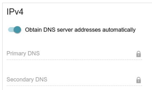
Figure 81. The page for creating a new PPPoE Pv6 connection. The IPv4 section.
