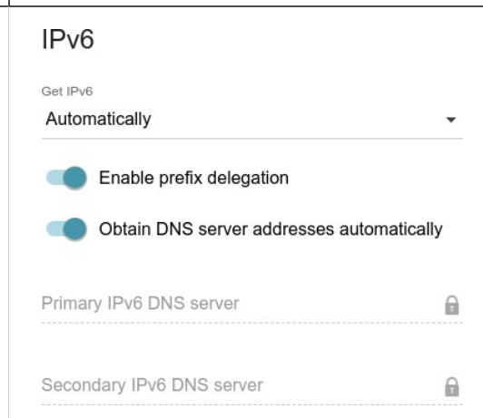
Figure 82. The page for creating a new PPPoE Pv6 connection. The IP section.
