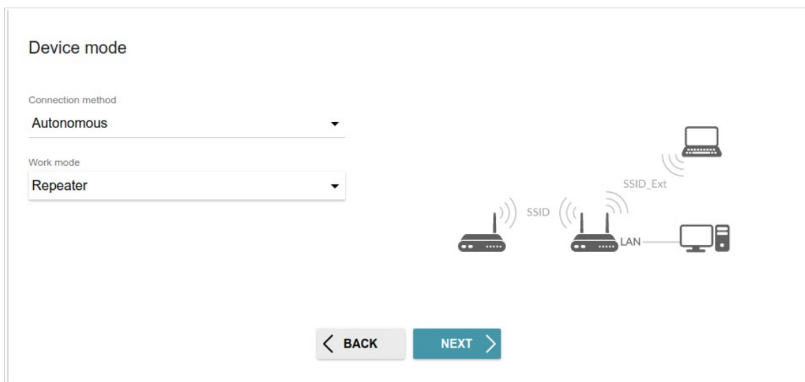
Figure 40. Selecting an operation mode. The Repeater mode.
