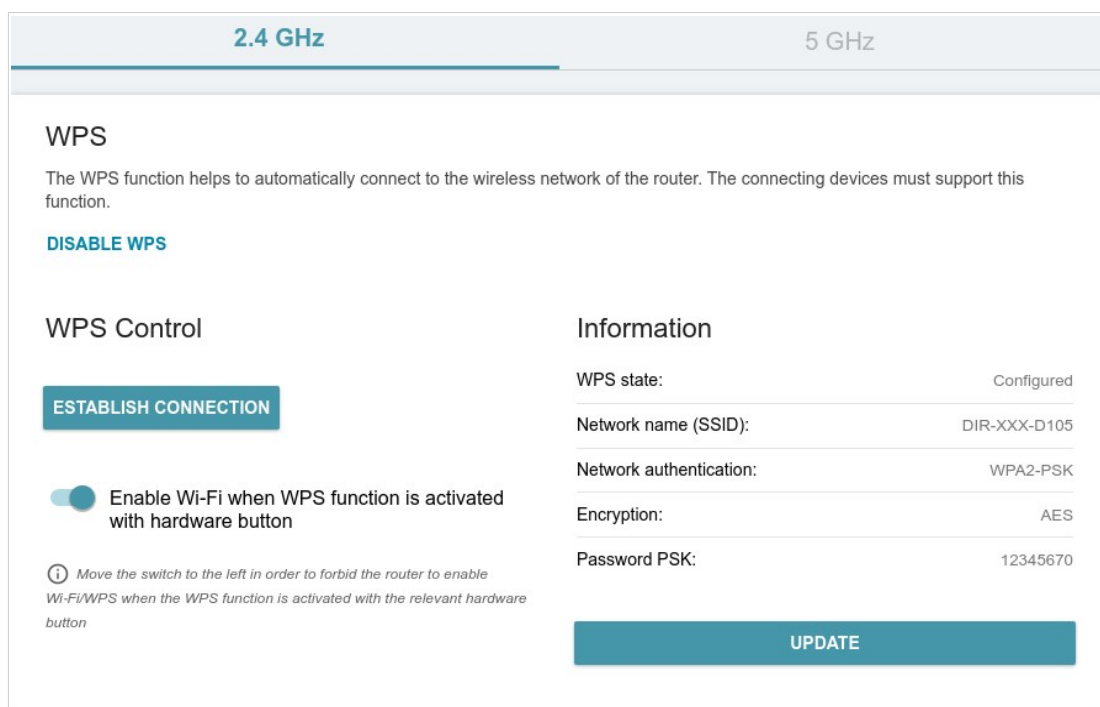
Figure 135. The page for configuring the WPS function.
