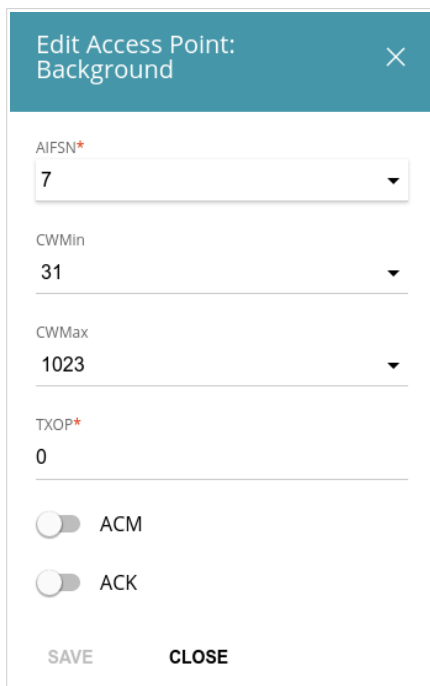
Figure 137. The window for changing parameters of the WMM function.
