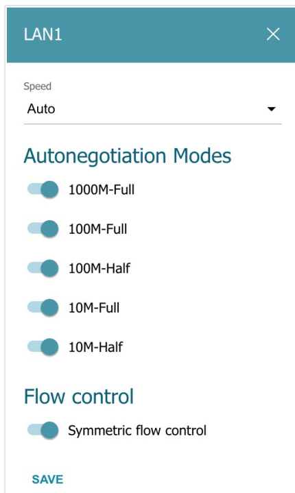
Figure 161. The window for changing the settings of the router's port.
