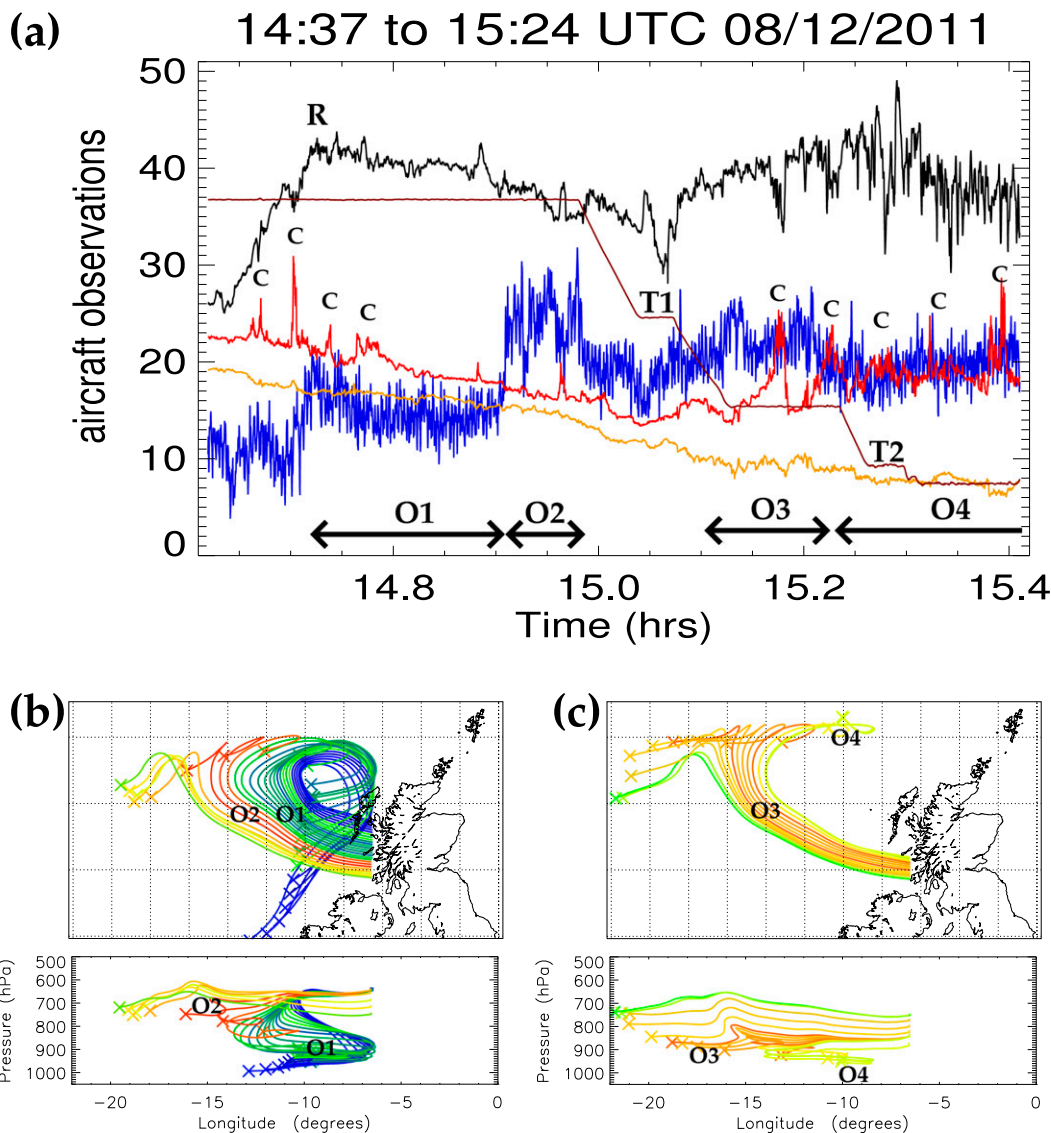
FIG. 7. (a) Time series from FAAM aircraft on low-level legs through the strong wind region showing that black is wind speed ( \text{m s}^{-1} ); blue is \text{CO} - 100 (ppbv); orange is \theta ( ^{\circ}\text{C} ); red is \theta_e ( ^{\circ}\text{C} ); and dark red is 0.01z (m). Observed air masses are labeled O1, O2, O3, and O4 using CO as a guide. Location R is the edge of warm seclusion at radius of maximum winds; T1 is the turn at southern end of flight track; T2 is the second turn; and C is the observed cloud band. (b) Back trajectories (1.125 days long) calculated with ERA-Interim winds from points at 1-min intervals along the aircraft track heading southward from the beginning of the time series to turn T1. (c) Back trajectories (1.25 days) from the track heading northward from turn T1 to T2. The trajectories are colored by observed CO (using the same scale).
