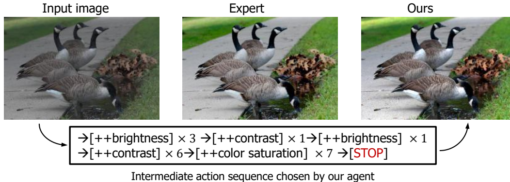
Figure 1. One example of our method. Using deep reinforcement learning, we train our agent with human expert’s images in MIT-Adobe FiveK dataset [1]. The agent iteratively selects an editing operation to apply and automatically produces a retouched image with an interpretable action sequence.
