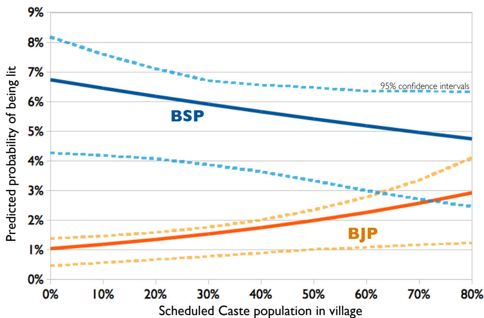
Figure 6: Predicted probability of being newly lit in BSP constituencies
