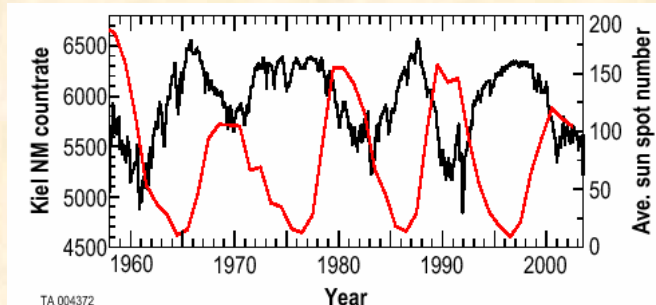
Figure FO1-1. Ground-based neutron monitor observations (black) provide a proxy for GCR flux. (Sunspot number is in red). GCRs are modulated by solar activity with a 15-30% reduction at solar maximum.
