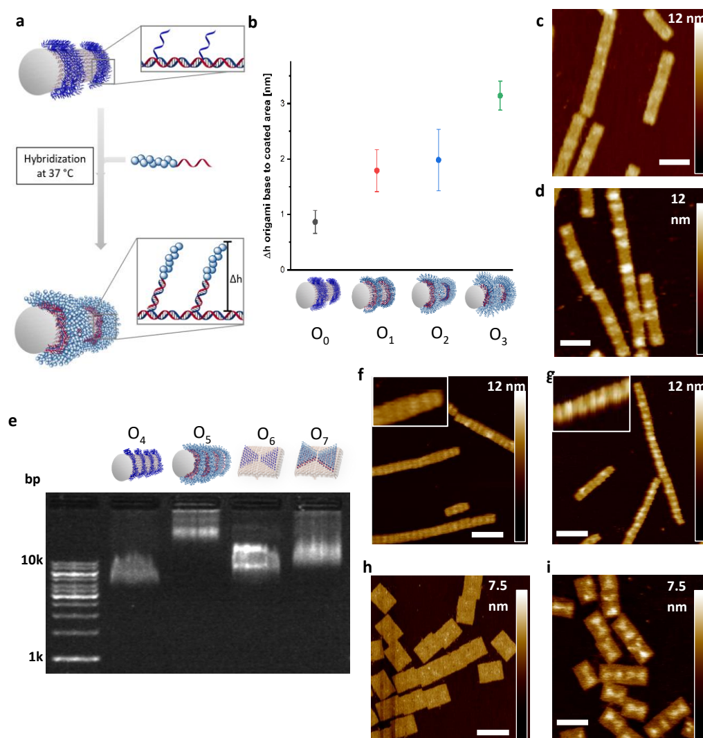
Figure 3: a) Schematic representation of the DNA-origami coating with DNA-polymer conjugates by hybridization at 37 °C. b) Height changes of the DNA origami surface obtained via AFM, where the respective uncoated and the coated sections on the origami nanostructures were measured to obtain the height difference ( n=10 times for each coating). Heights from Figure S5-S8 and Table S4-S7 c) Uncoated DNA-origami imaged by AFM. Scale bar = 80 nm. d) DNA-origami coated with CP3 imaged by AFM. Scale bar = 80 nm. e) Monitoring of the coated and uncoated DNA-origami tube and rectangle containing StA by 1% agarose gel, stained with SYBR Gold; L: DNA ladder; O 4 : uncoated DNA-origami; O 5 : coated DNA-origami with CP3; O 6 : uncoated DNA-origami; O 7 : coated DNA-origami with CP2. f-i) Respective DNA-origami architectures uncoated and coated with the respective DNA-polymer conjugate; tube: CP3; rectangle: CP2. Scale bar = 120 nm.
