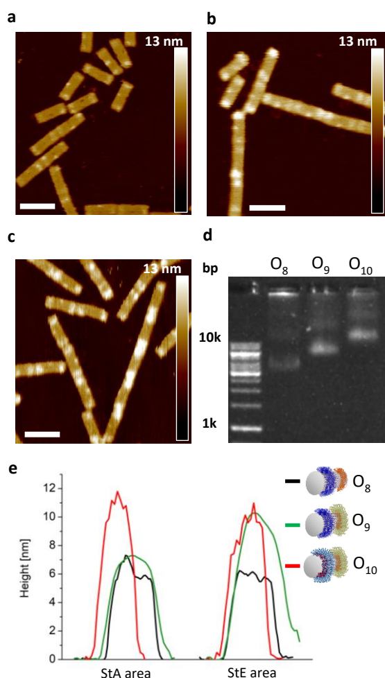
Figure 4: a) Uncoated DNA-origami ( O 8 ) monitored via AFM. Scale bar = 100 nm b) DNA-origami ( O 9 ) with StE C -P7 monitored via AFM. Scale bar = 100 nm c) DNA-origami ( O 10 ) coated with StE C -P7 and CP2. Scale bar = 100 nm d) Coated and uncoated DNA-origami monitored with 1% agarose gel, stained with SYBR Gold. O 8 is uncoated, O 9 is coated with StE C -P7 and O 10 is coated with CP2 and StE C -P7. e) AFM topographic images reveal a significant increase in height of the respective coating area.
