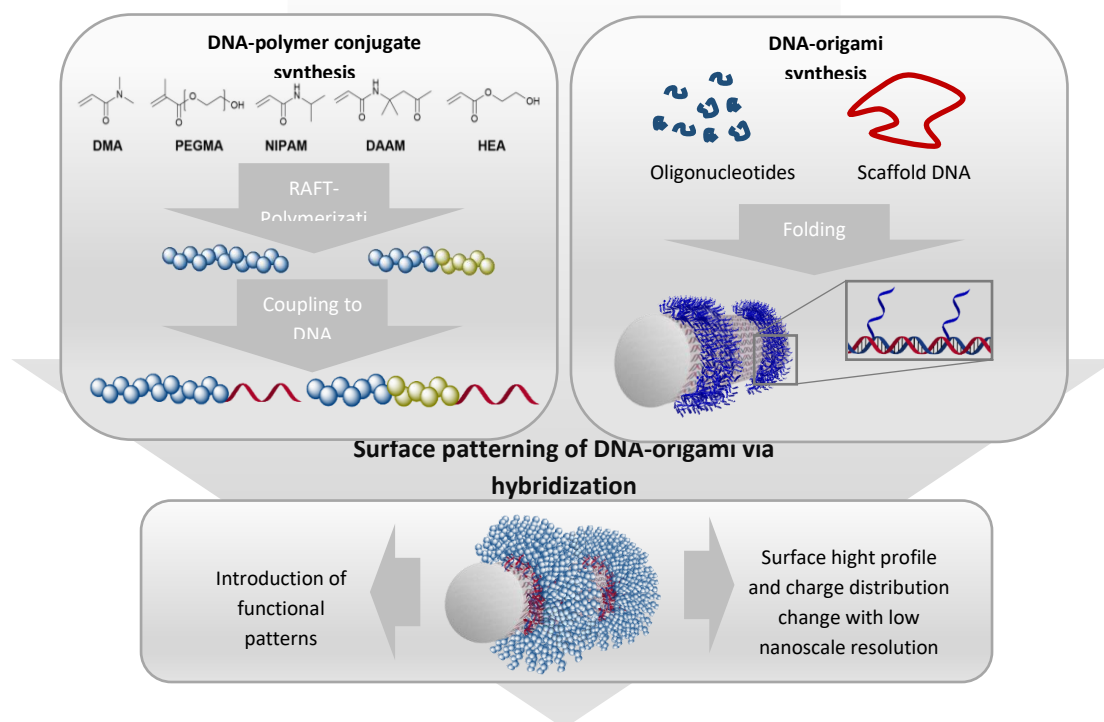
Figure 1: Concept of the combination of the grafting to method for generating DNA-polymer conjugates and the surface coating of DNA-origami due to protruding single stranded sticky sequences on the surface. The selected monomers form polymers with different features to diversify the inherent properties of DNA-origami nano-objects. The monomers were polymerized via RAFT polymerization and then coupled to single stranded DNA via NHS-amine conjugation chemistry under mild and ambient conditions. This versatile method generates a wide range of DNA-polymer conjugates for precise surface patterning of DNA-origami nanostructures.
