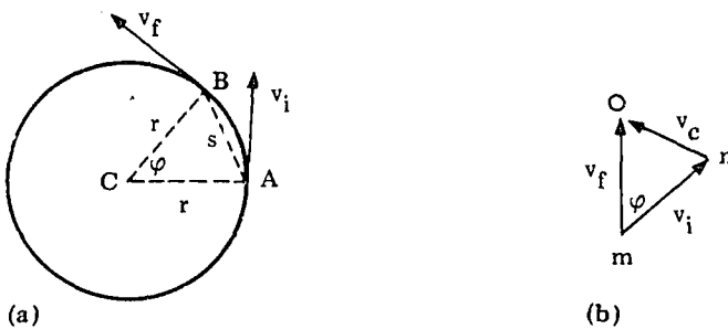
Figure 2-2 Velocity Vectors
