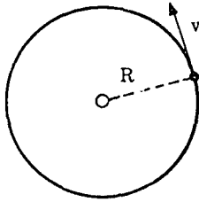
Figure 2-1 Uniform Circular Motion
