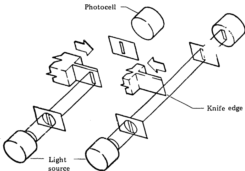
Figure 3-2 Photodetector Principle
