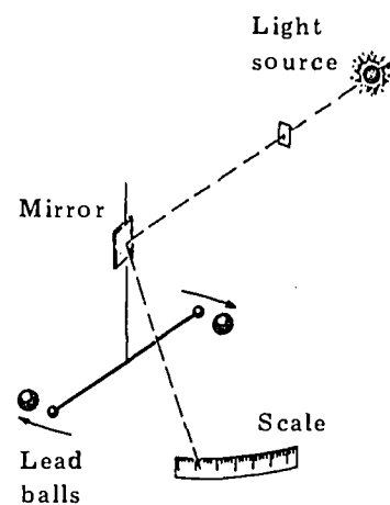
Simplified drawing of the Cavendish experiment. By observing the deflection of the light beam, the gravitational attraction between the lead balls can be measured.
