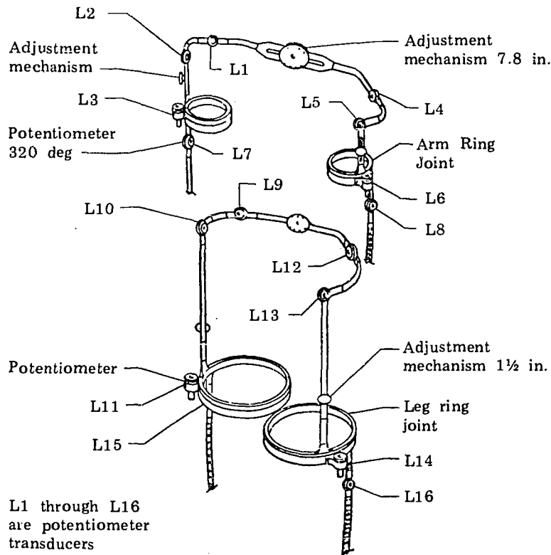
Figure 4-3 Exoskeletal Structure
