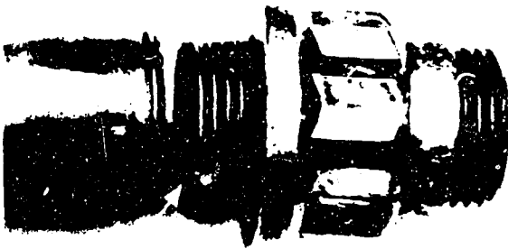
A COMPLETE THREAD ROOT FAILURE
