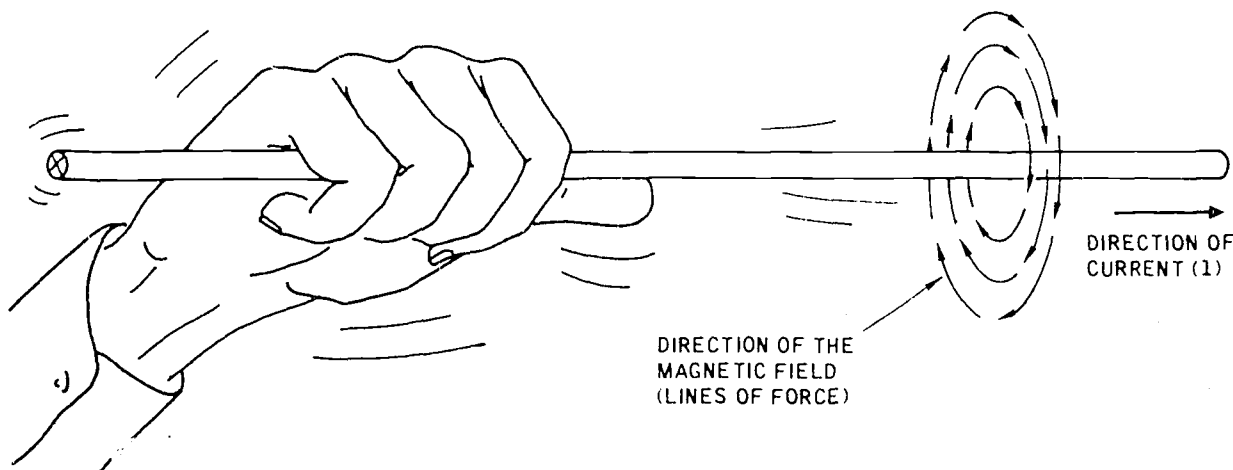
Figure 2-9. Right-Hand Rule
