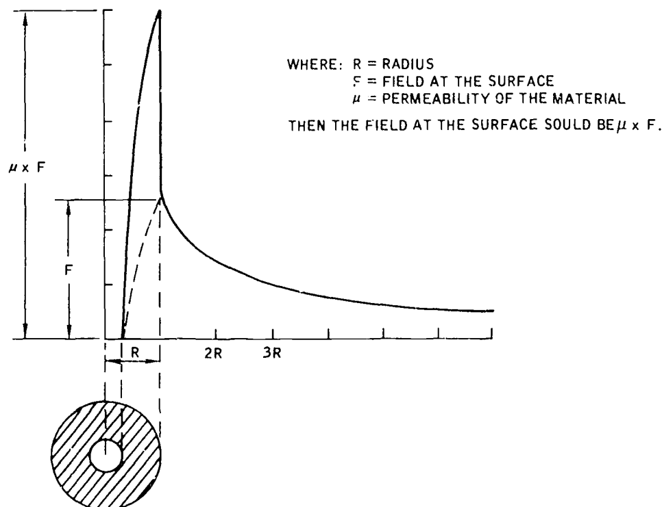
Figure 2-18. Field Distribution In and Around a Hollow Magnetic Conductor
