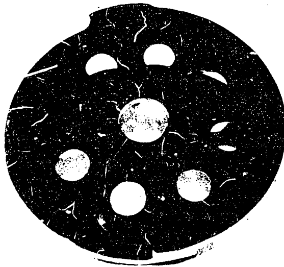
Figure 6-10. Heat Treat Cracks
