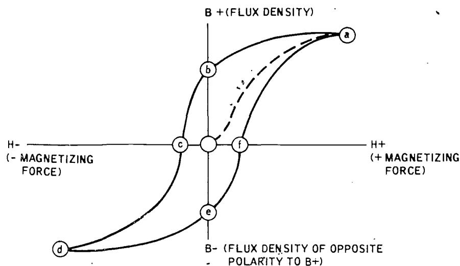
Figure 2-11. The Hysteresis Curve
