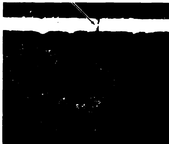
C HYDROGEN EMBRITTLEMENT PROPAGATED THROUGH CHROME PLATE
