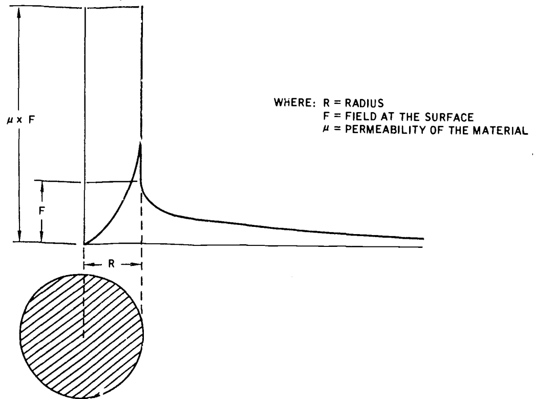
Figure 2-20. Field Distribution In and Around Solid Magnetic Conductor Carrying Alternating Current
