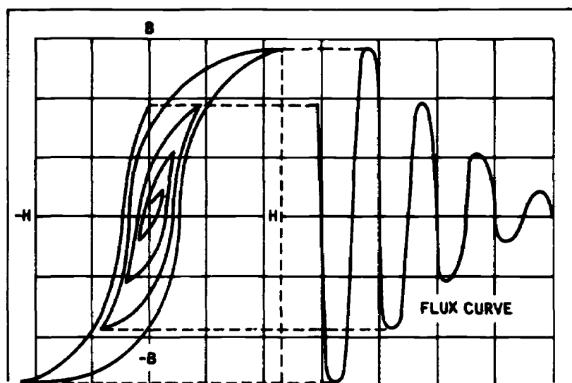
Figure 2-26. Demagnetization Flux-Curve Projected from Hysteresis Curve
