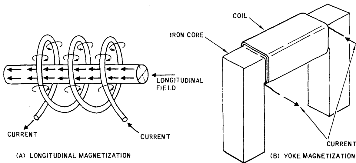
Figure 2-14. Longitudinal Magnetization
