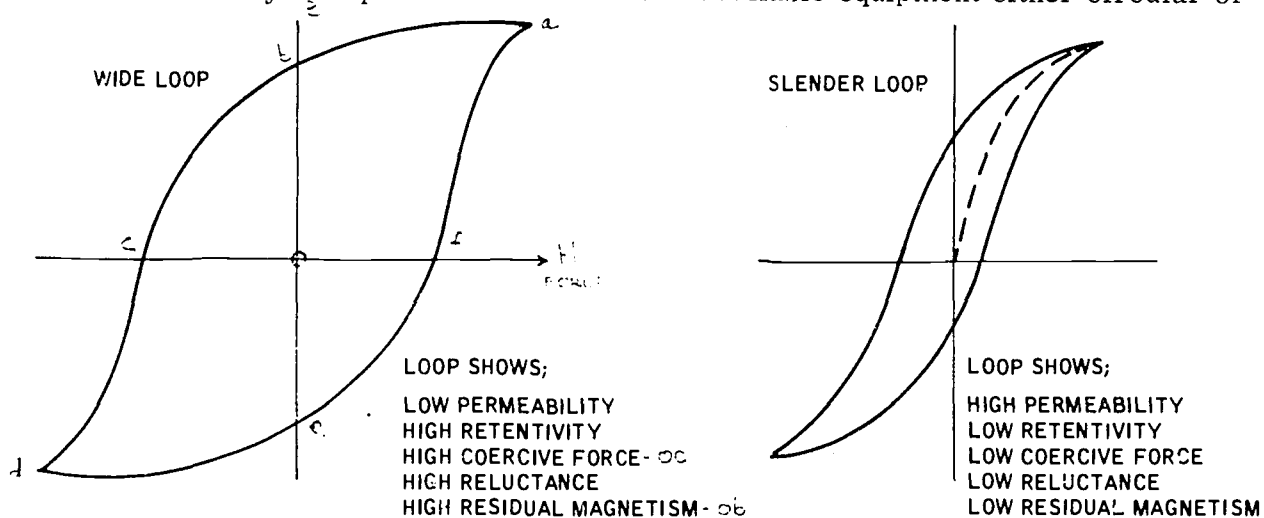
Figure 2-12. Hysteresis Loop Characteristics
