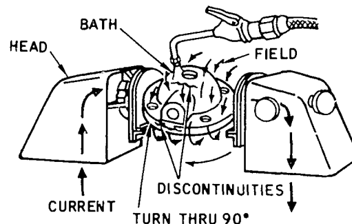
SHOT NO. 3 — SECOND HEAD SHOT ACROSS A DIAMETER
