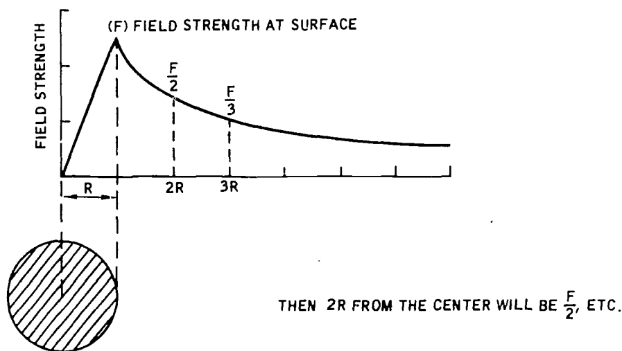
Figure 2-15. Field Distribution In and Around a Nonmagnetic Conductor
