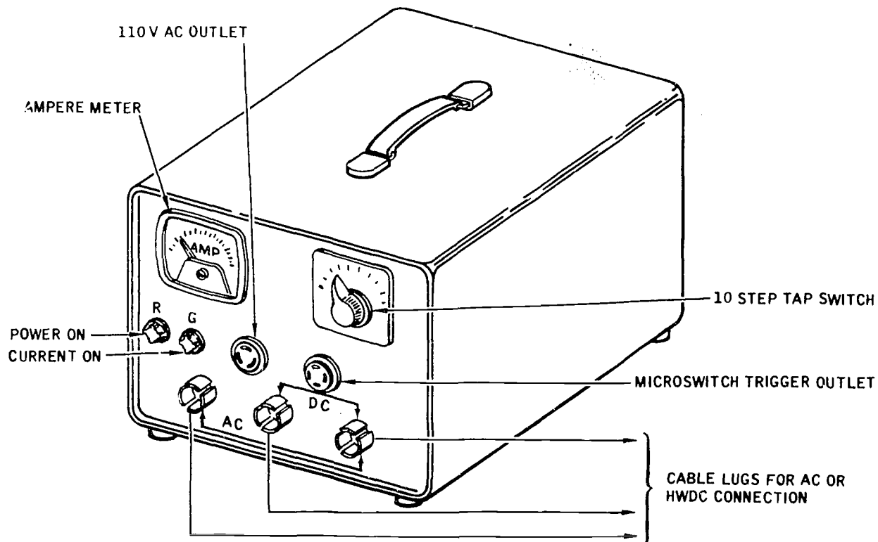
Figure 3-3. Portable Magnetic Particle Test Equipment
