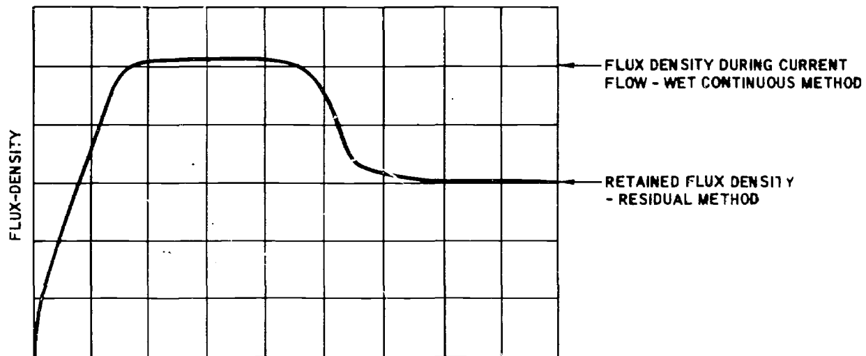
Figure 5-11. Flux Density Curve
