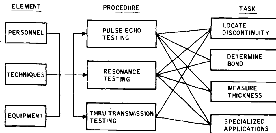
Figure 7-3. Ultrasonic Test
