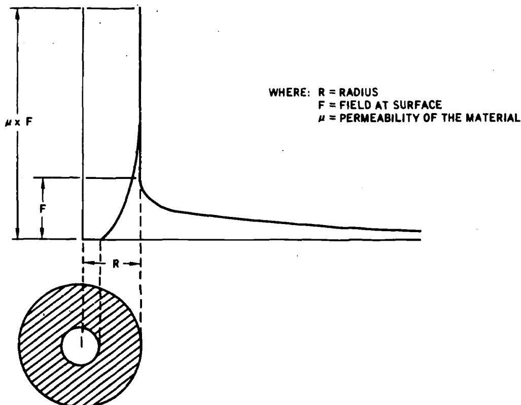
Figure 2-21. Field Distribution In and Around a Hollow Magnetic Conductor Carrying Alternating Current
