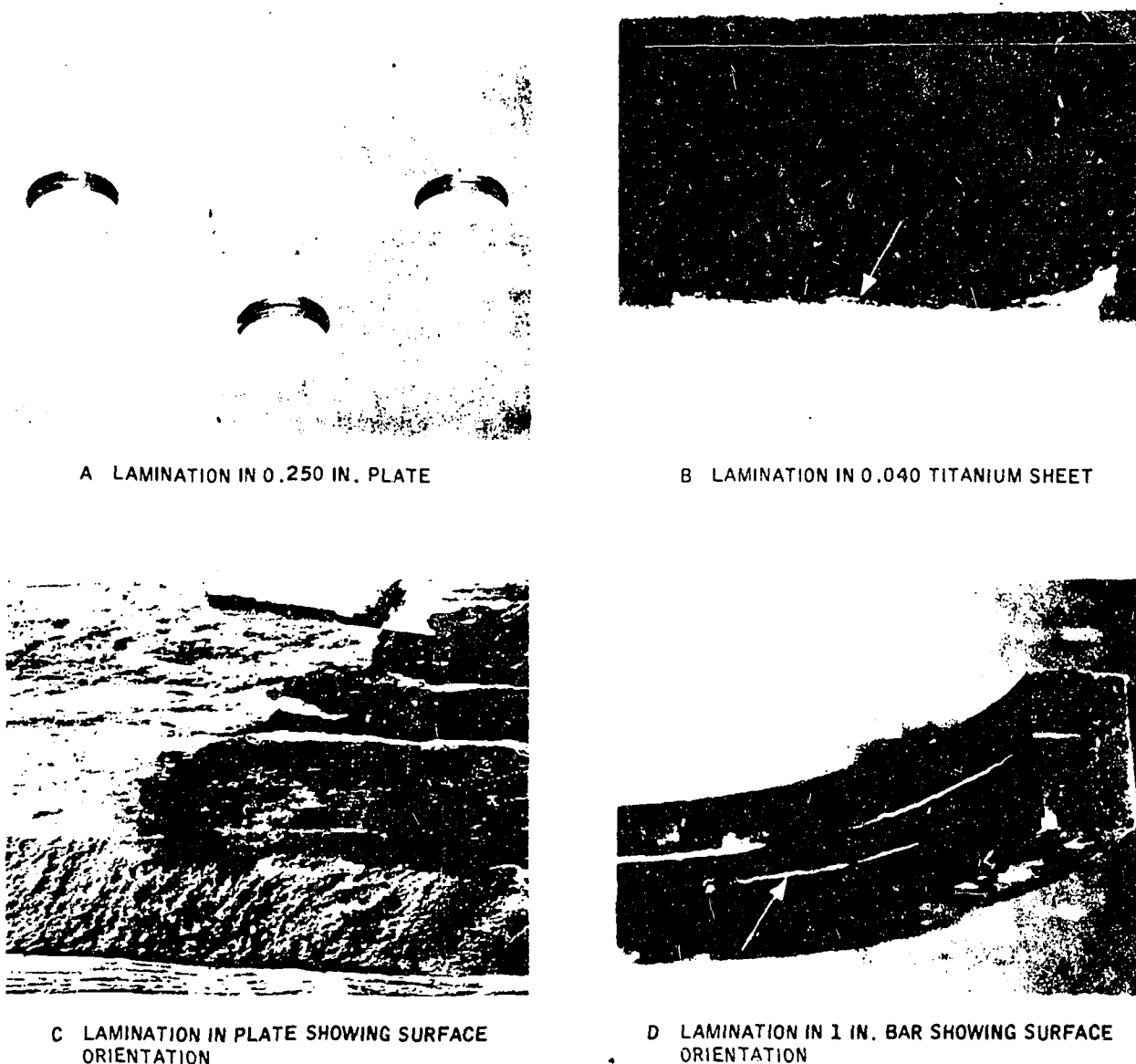
Figure 7-21. Lamination Discontinuity
