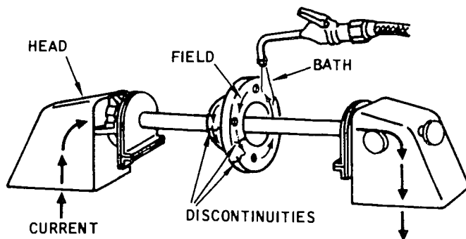
SHOT NO. 1 — HEAD SHOT (WITH CENTRAL CONDUCTOR)
