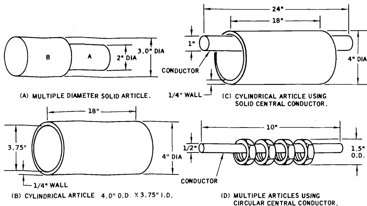
Figure 2-25. Circular Magnetization of Typical Specimens Using Head-Shot or Central Conductor
