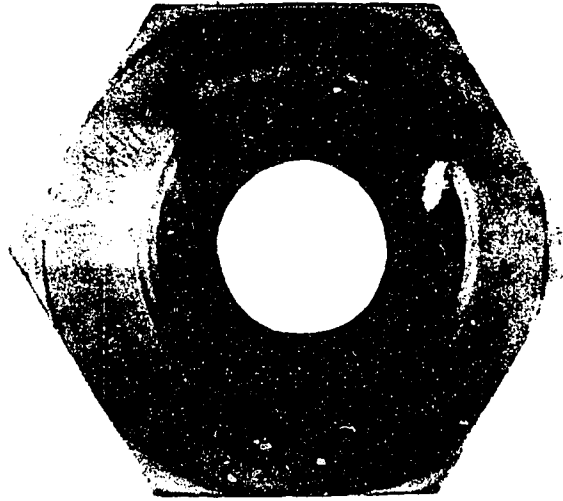
Figure 6-9. Grinding Cracks
