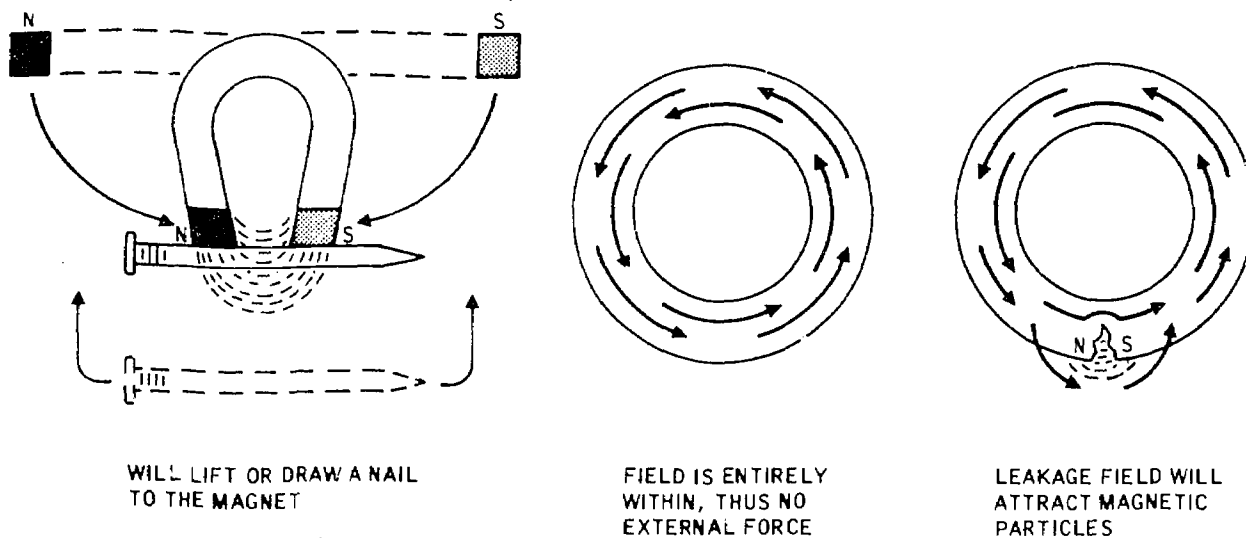
Figure 2-4. Poles in Straight Bar, Horseshoe, and Broken Magnet
