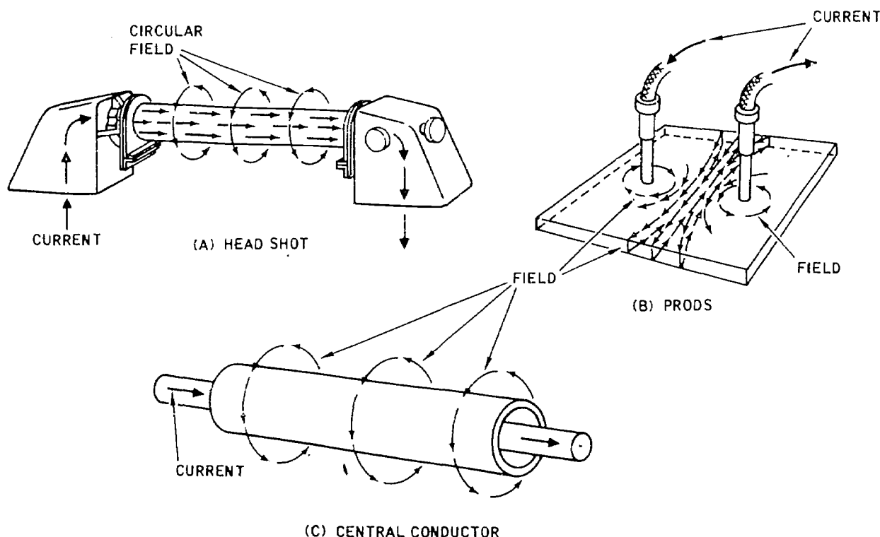
Figure 2-13. Circular Magnetization by Direct and Indirect Current Induction
