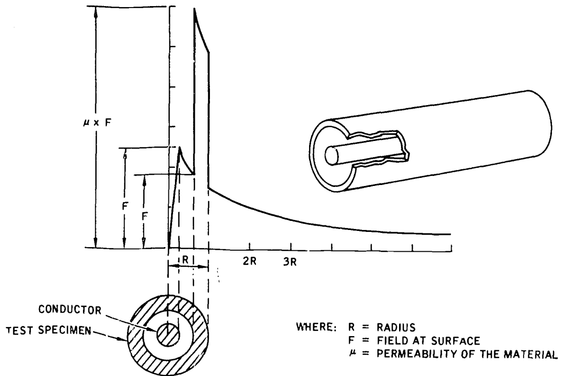
Figure 2-19. Field Distribution In and Around a Hollow Magnetic Cylinder With Central Conductor
