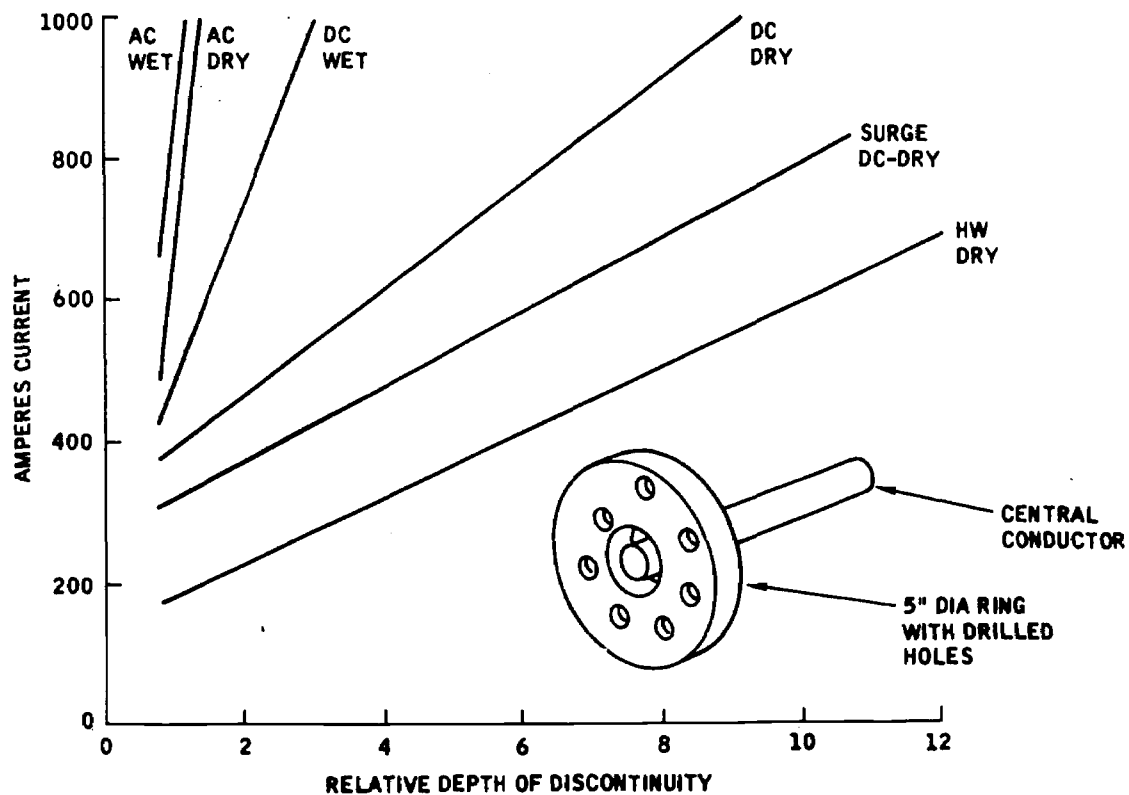
Figure 2-24. Threshold Sensitivities of Various Metals
