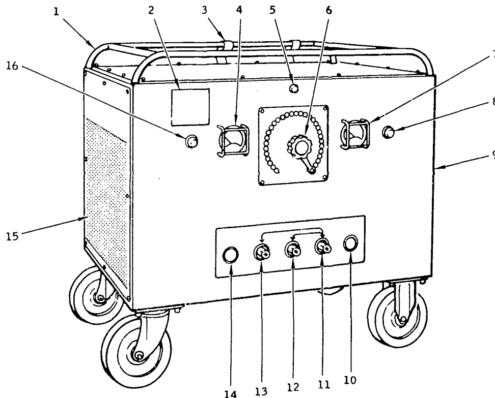
Figure 3-2. Mobile Magnetic Particle Test Equipment
