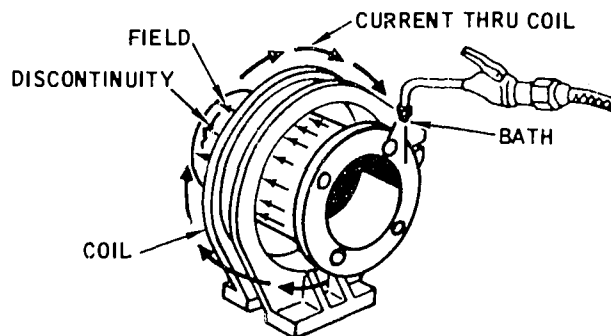
Figure 5-6. Magnetization of Irregularly Shaped Specimens
