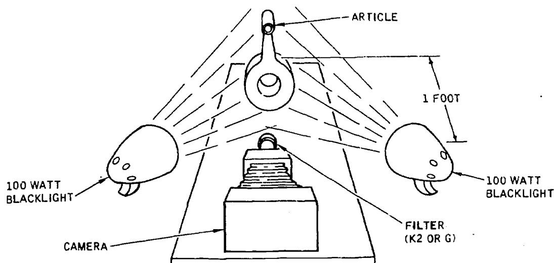
Figure 6-12. Photographing Fluorescent Indications
