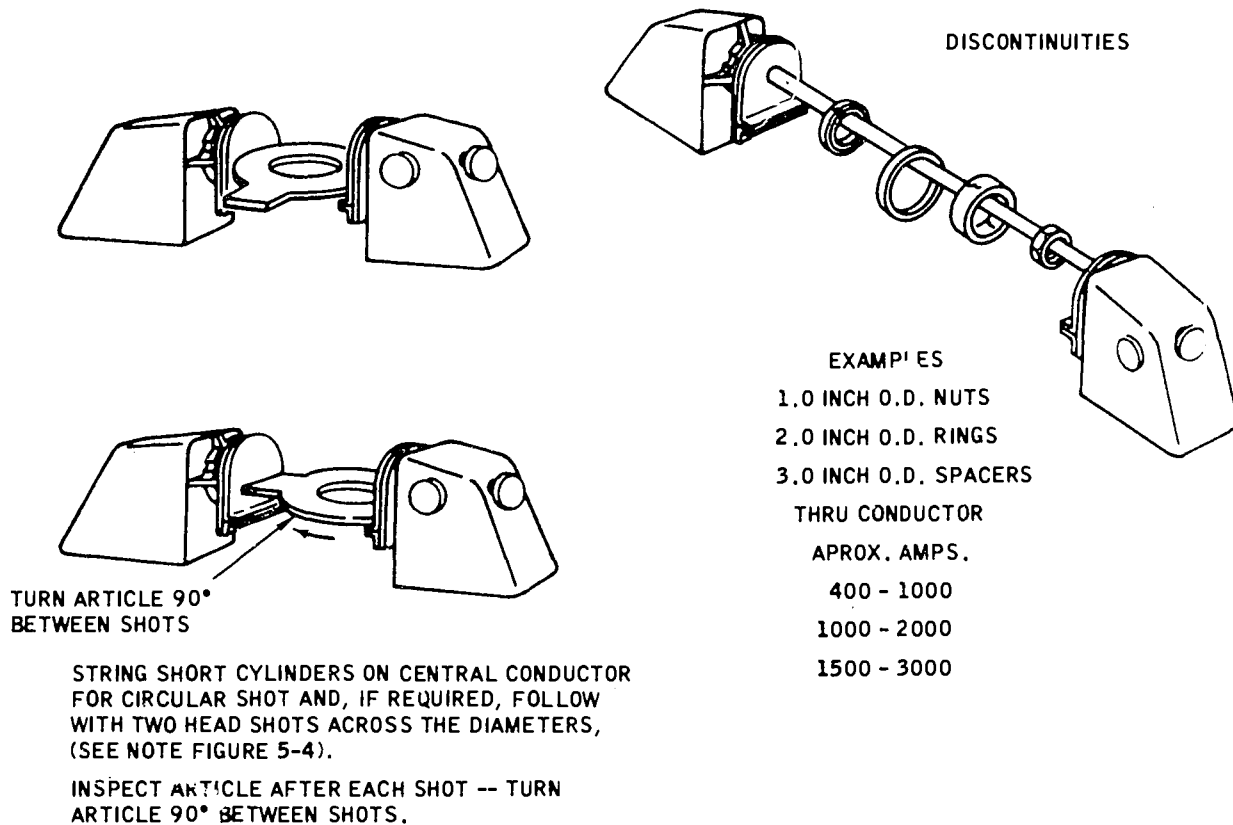
Figure 5-4. Magnetization of Very Short Hollow Cylinders
