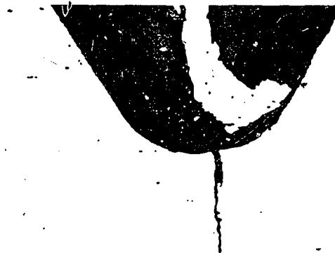
D MICROGRAPH OF (B) SHOWING TRANSGRANULAR CRACK AT THREAD ROOT
