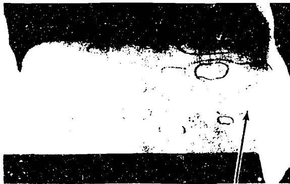
B STEEL FORGING SHOWING NUMEROUS INCLUSIONS
