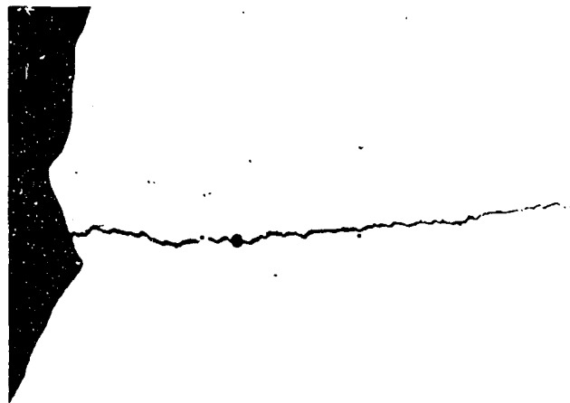
B MICROGRAPH OF CRACK SHOWN IN (A)
