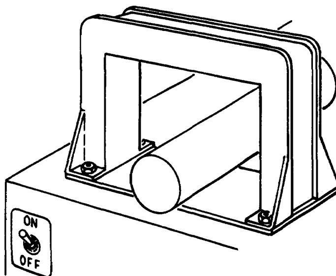
Figure 2-27. Demagnetization Coil
