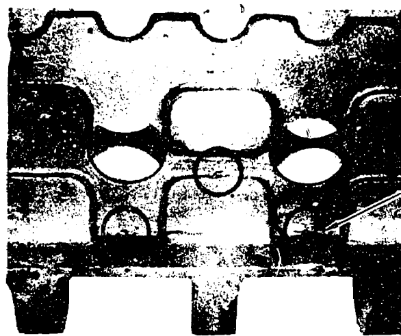
B HOT TEARS IN FILLET OF CASTING
