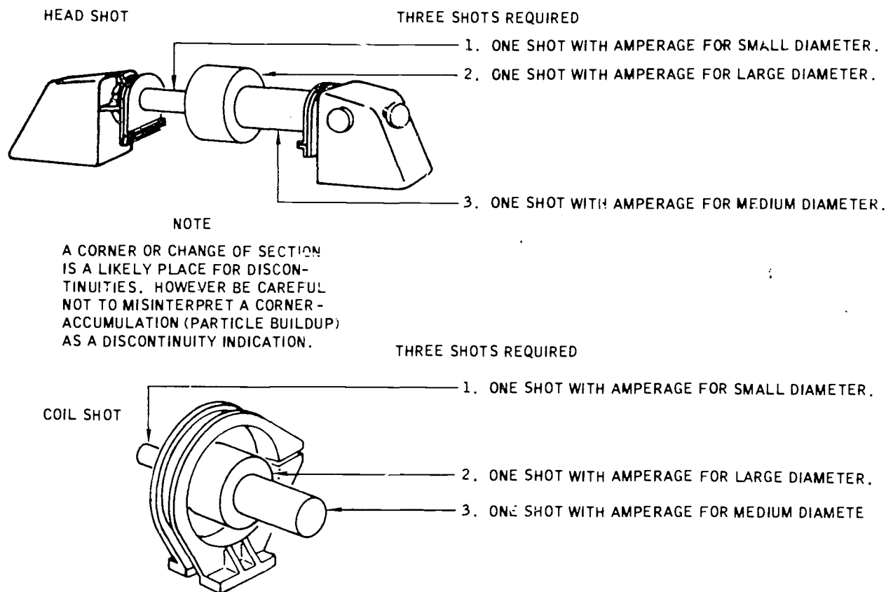
Figure 5-2. Magnetization of Cylindrical Specimen w-Var: Diameter
