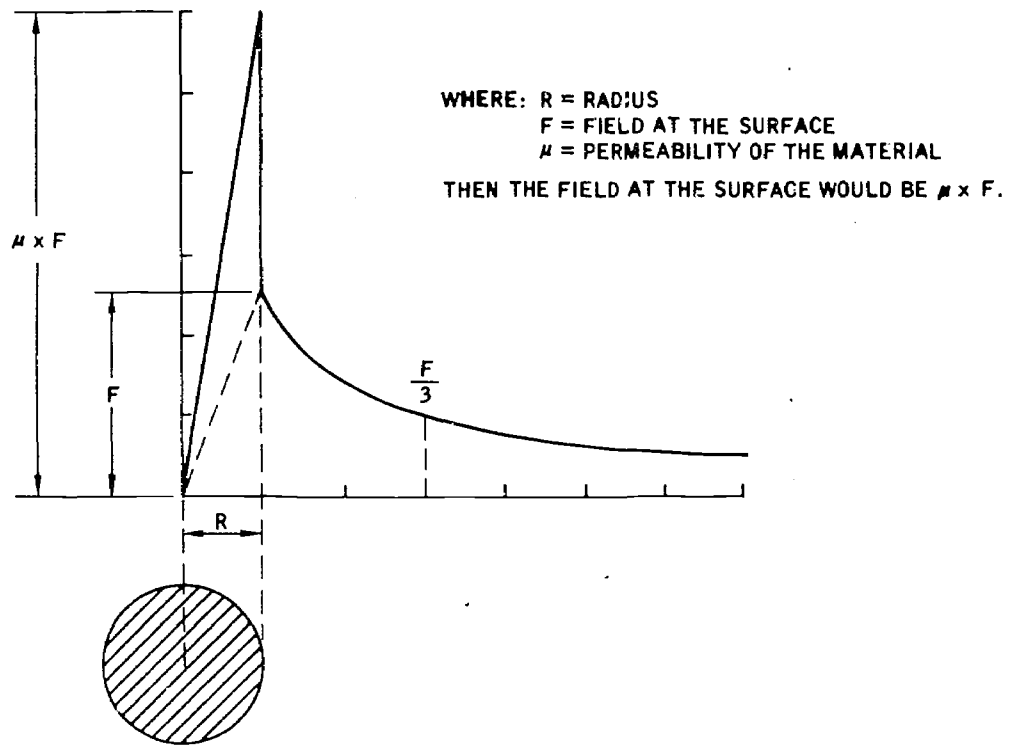
Figure 2-16. Field Distribution In and Around a Solid Magnetic Conductor
