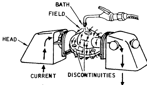
SHOT NO. 2 — FIRST HEAD SHOT ACROSS A DIAMETER
