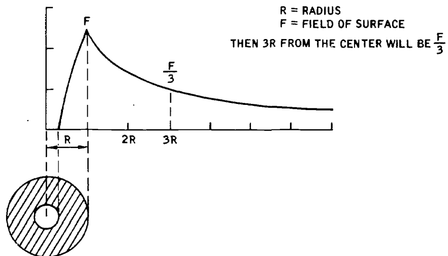
Figure 2-17. Field Distribution In and Around a Hollow Nonmagnetic Conductor
