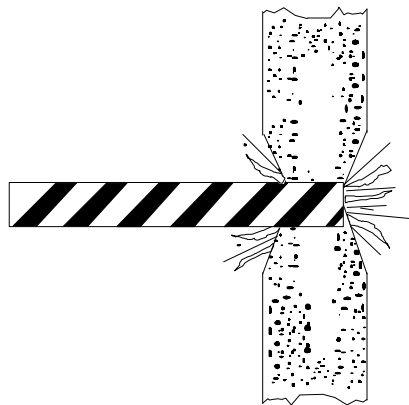
(b) Target scabbing
