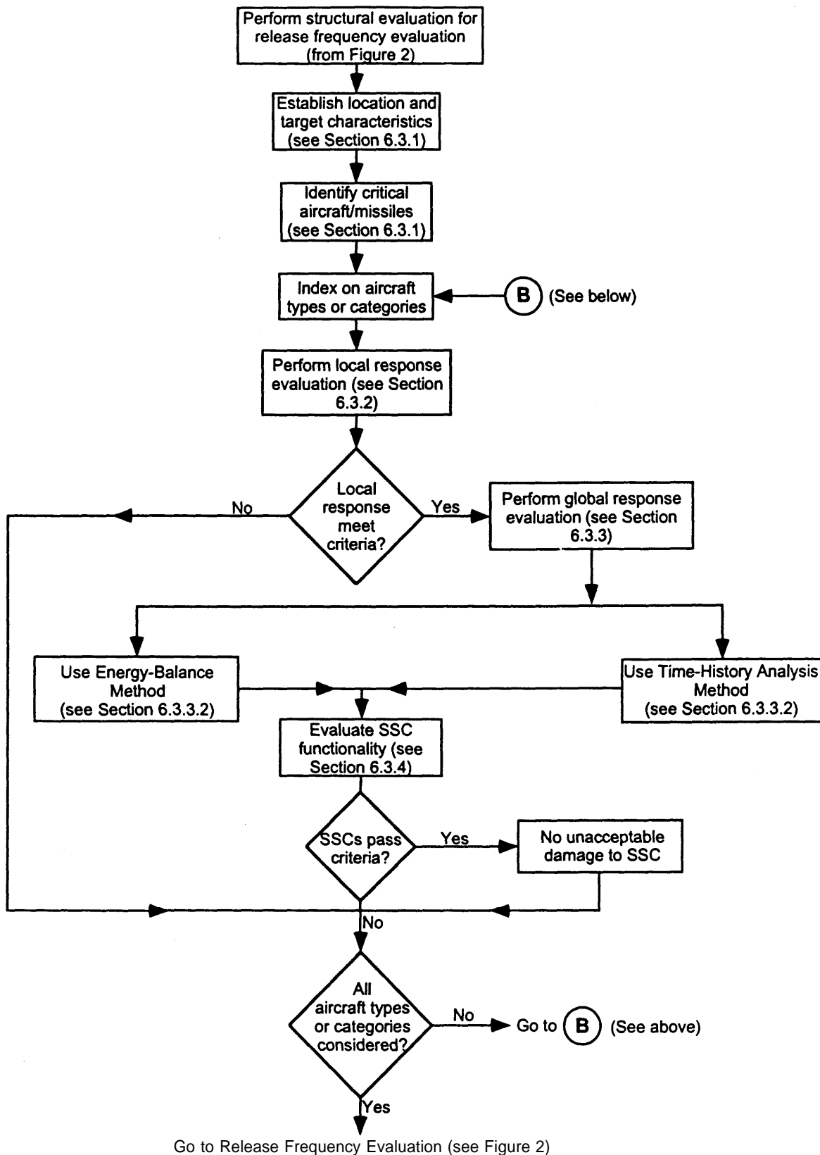
Figure 2b: Structural Evaluation for Release Frequency Evaluation
