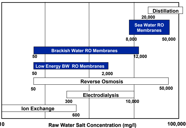
Figure 1.1 Major desalination processes
