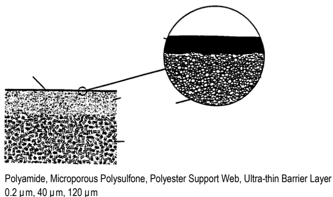
Figure 1.10 Schematic cross-section of a FILMTEC thin-film composite membrane
