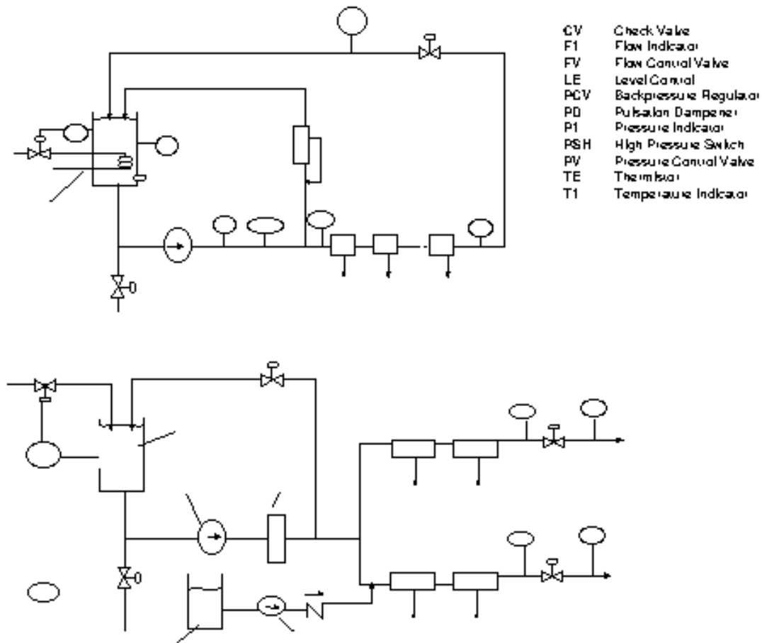
Figure 9.6 Flow schematic
