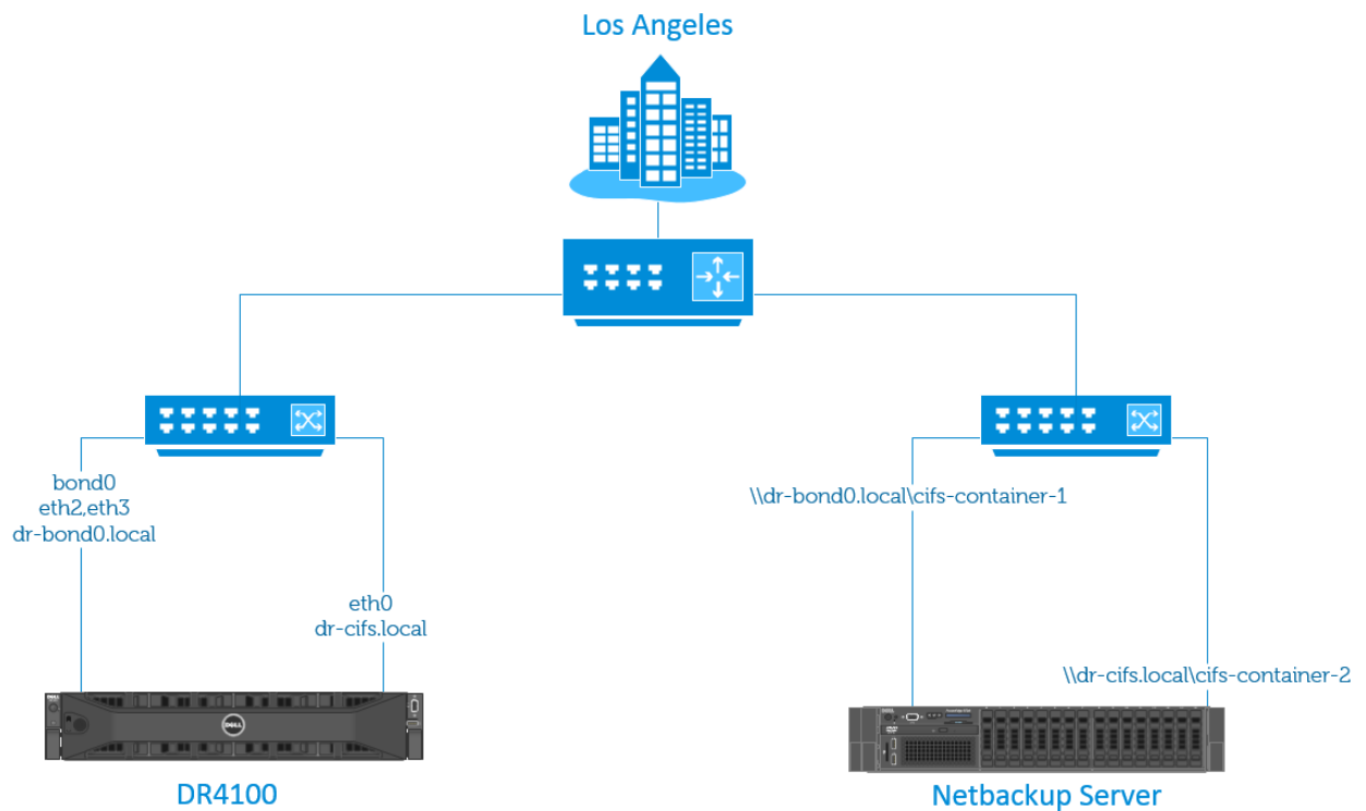
Figure 7 Scenario 5 topology
