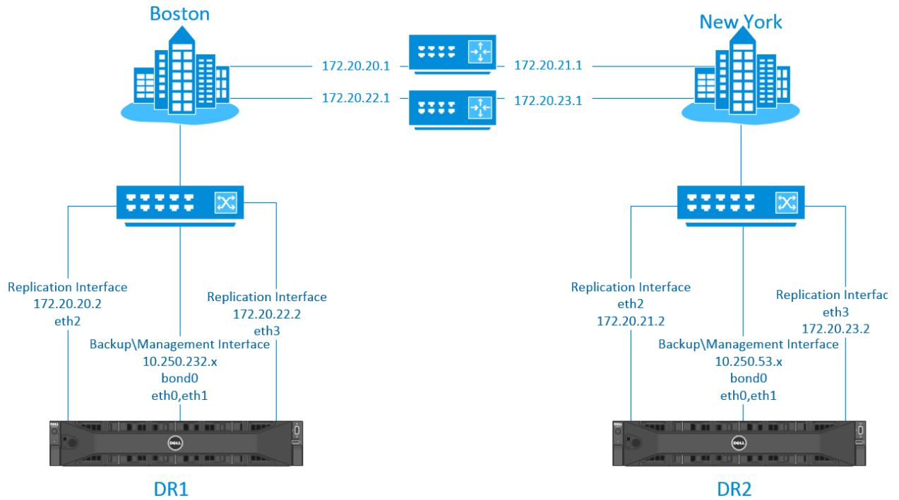
Figure 5 Scenario 3 topology
