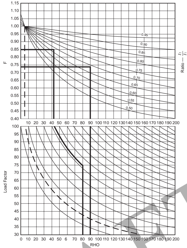
Figure B.310.15(B)(2)(1) Interpolation Chart for Cables in a Duct Bank I_1 = ampacity for Rho = 60, 50 LF; I_2 = ampacity for Rho = 120, 100 LF ( load factor); desired ampacity = F \times I_1 . [ROP 6-202]
