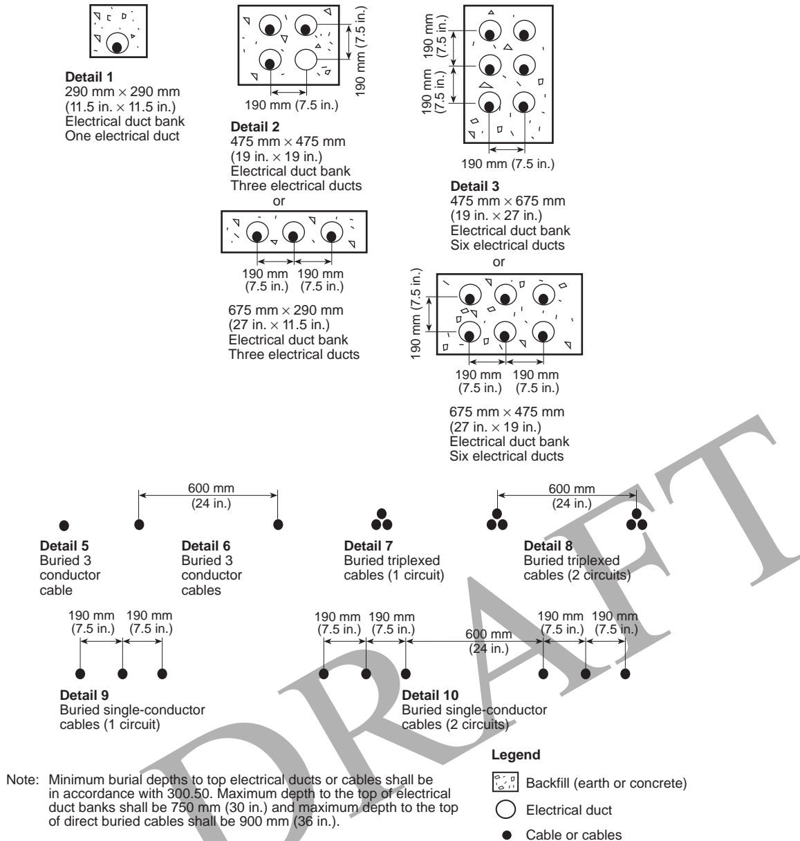
Figure 310.60 Cable Installation Dimensions for Use with Table 310.60(C)(77) Through Table 310.60(C)(86). [ROP 6-123]
