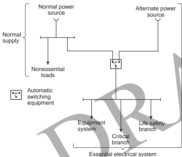
Informational Note Figure 517.30, No. 2 Hospital — Minimum Requirement (150 kVA or less) for Transfer Switch Arrangement. [ROP 15-70a]
