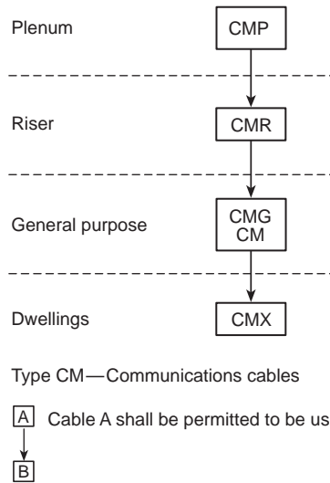
Figure 800.154 Cable Substitution Hierarchy. [ROP 16-172]
