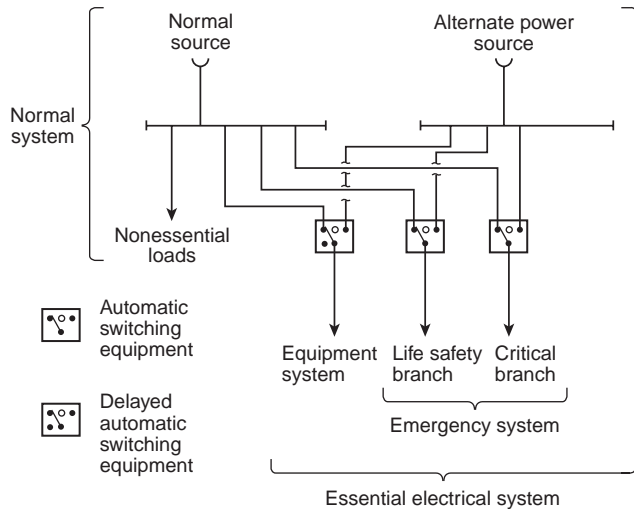
Informational Note Figure 517.30, No. 1 Hospital — Minimum Requirement (greater than 150 kVA) for Transfer Switch Arrangement. [ROP 15-69, 15-70a]
