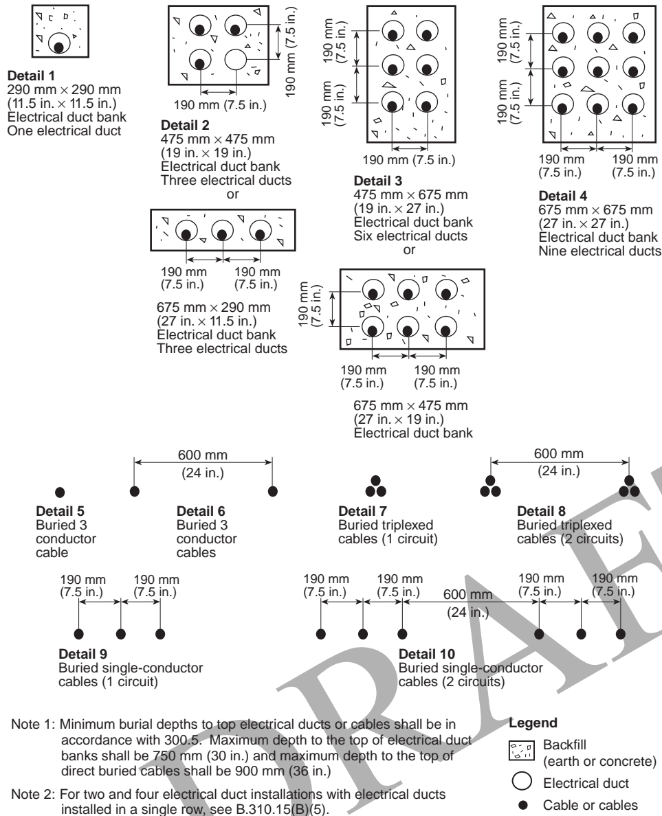
Figure B.310.15(B)(2)(2) Cable Installation Dimensions for Use with Table B.310.15(B)(2)(5) Through Table B.310.15(B)(2)(10). [ROP 6-202]
