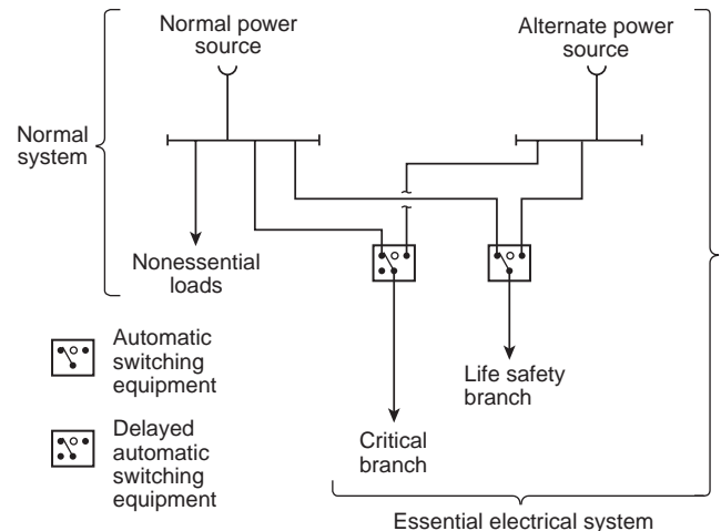
Informational Note Figure 517.41, No. 1 Nursing Home and Limited Health Care Facilities — Minimum Requirement (greater than 150 kVA) for Transfer Switch Arrangement. [ROP 15-104]
