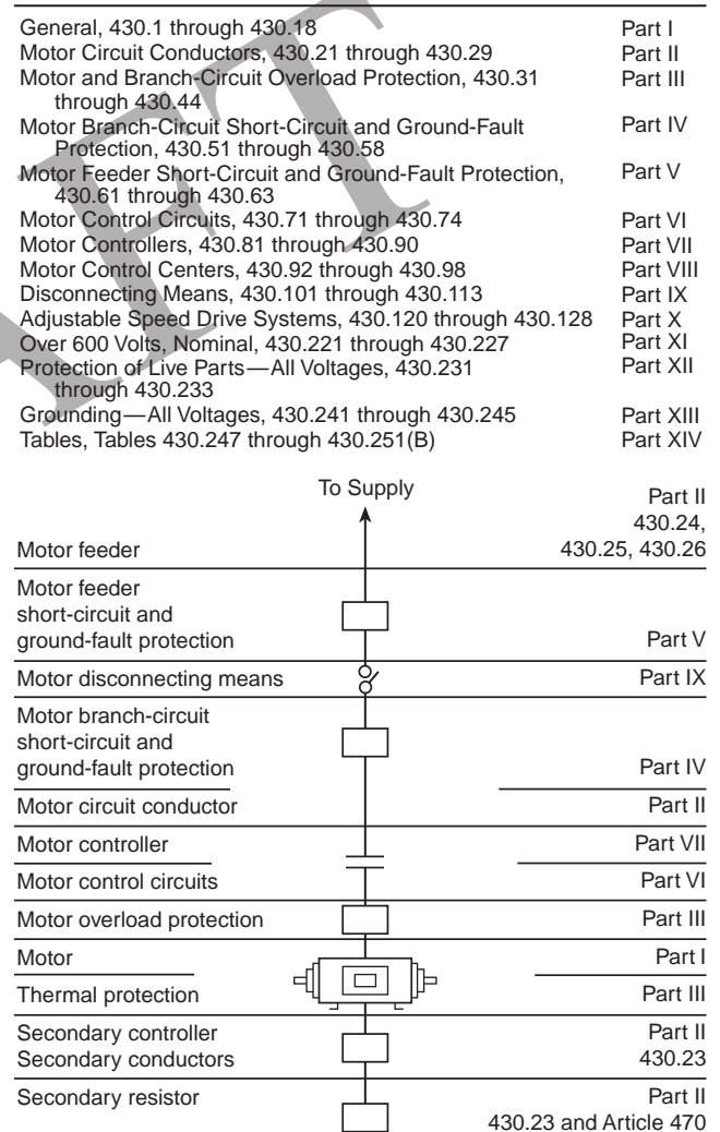
Figure 430.1 Article 430 Contents.
