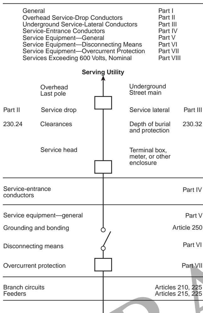
Figure 230.1 Services.
