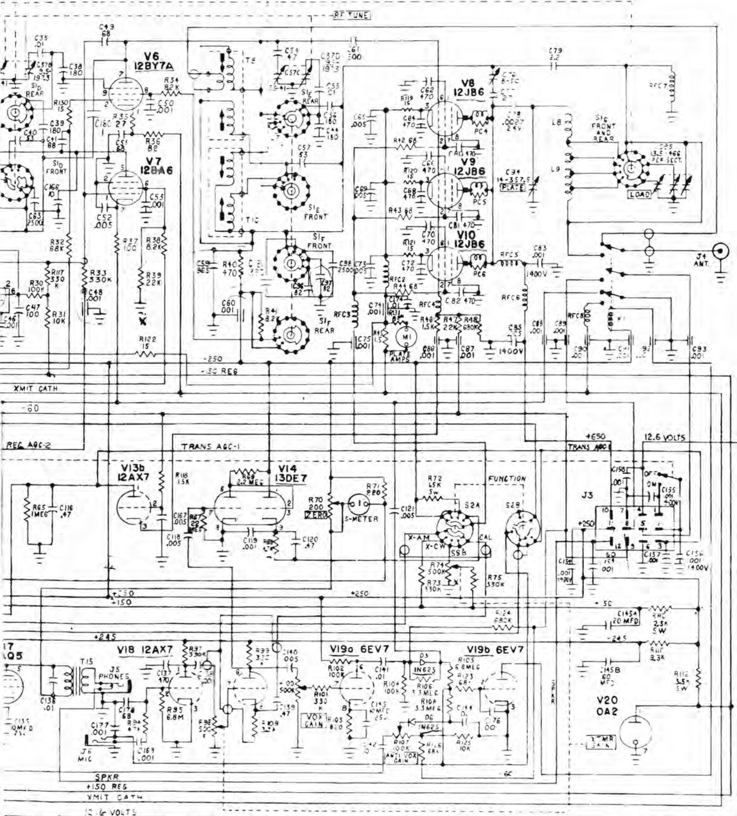
SCHMATIC DIAGRAM MODEL TR-3 SIDEBAND TRANSCEIVER
