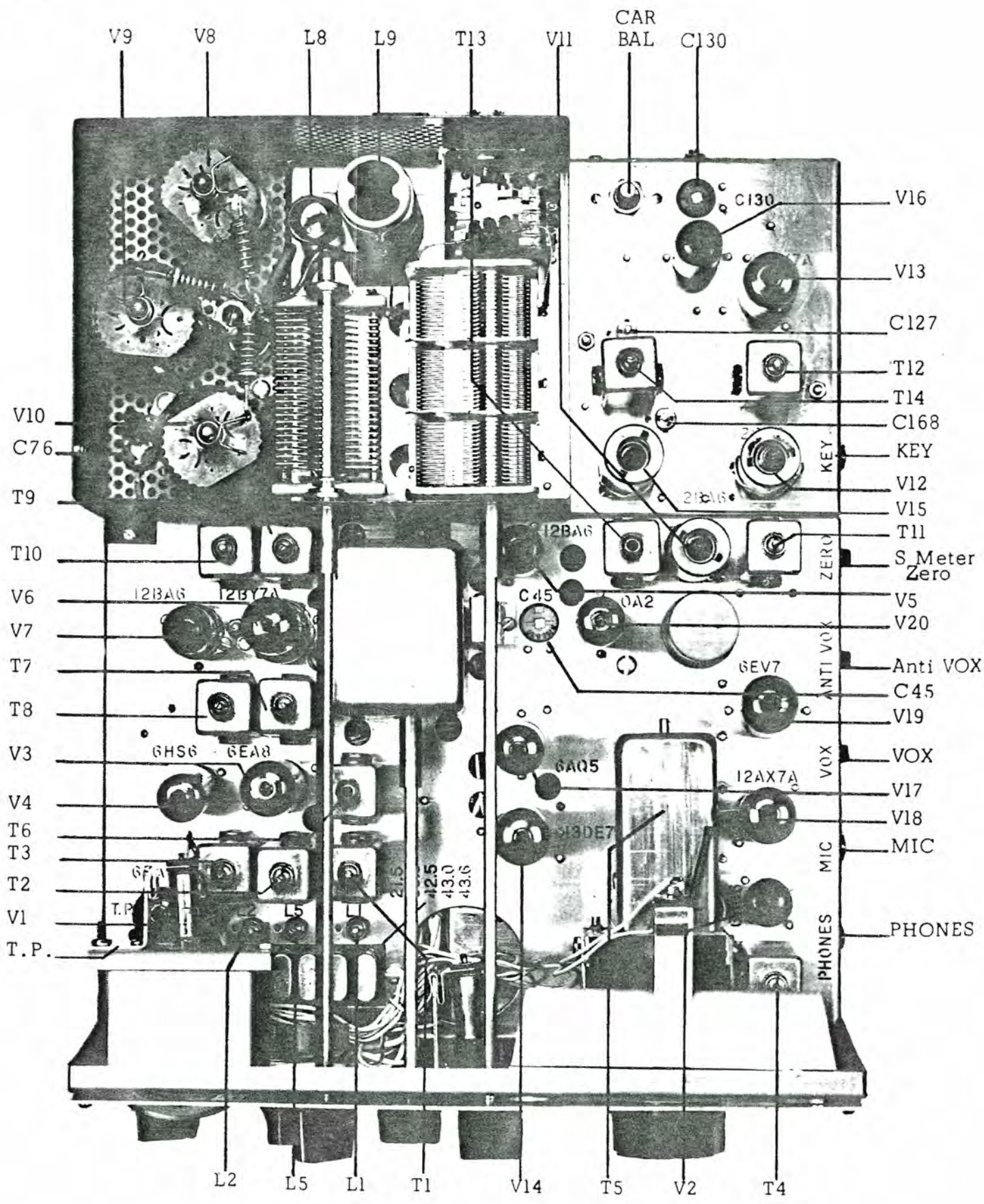
Figure 10 TOP VIEW
