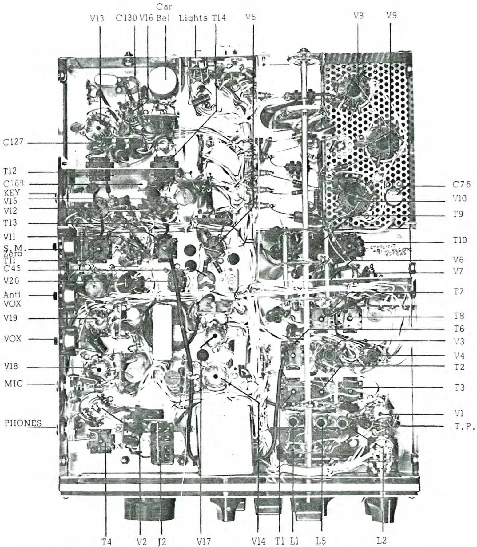
Figure 11 BOTTOM VIEW
