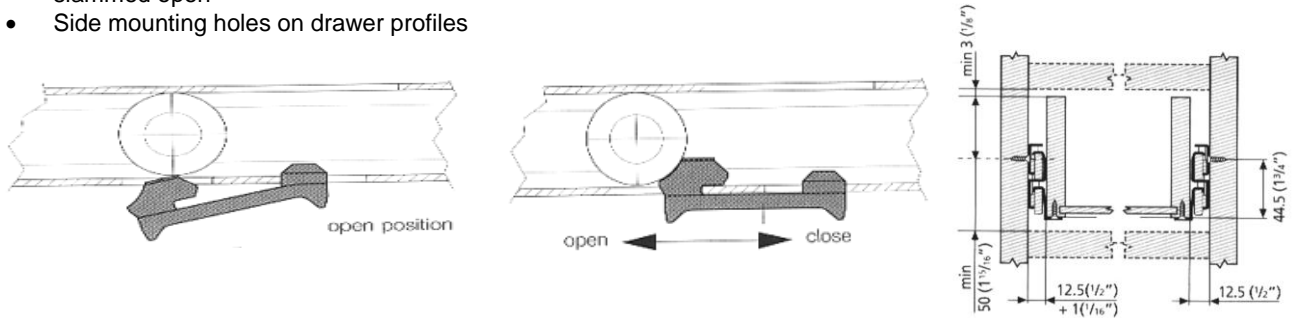
Illustration of function of impact absorbing stops and non-removable overrun safety clip. Moving down one 32mm hole spacing enables instant conversion to a regular-extension.
