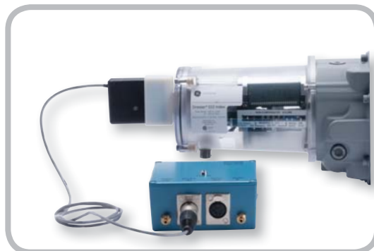
ES3 Prover Cable to Model 5 Prover Field Junction Box
