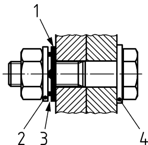
Figure 2 - Under Nut Fitting
