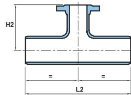
Spigot / Flange
