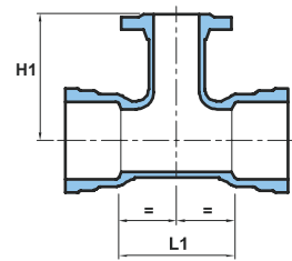
Socket / Flange
