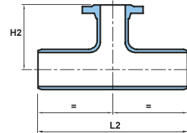
Spigot / Flange
