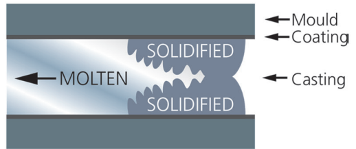
Figure 1: Directional Solidification
