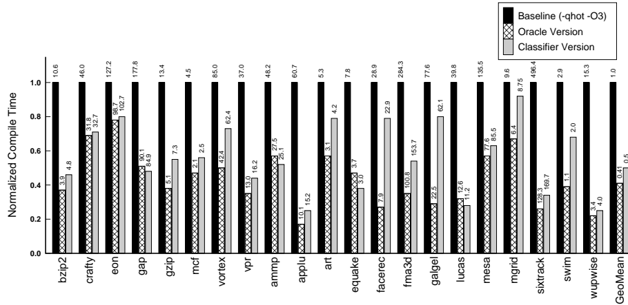
Fig. 4. Compile time comparison between the baseline, the oracle, and the classifier.
