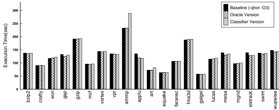
Fig. 5. Execution time comparison between the baseline, the oracle, and the classifier.
