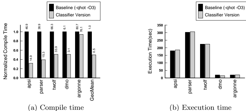
Fig. 6. Compile and execution time comparison for new benchmarks.
