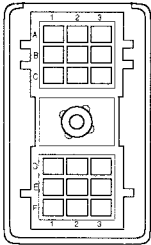
Vehicle Interface 18-way Connector
