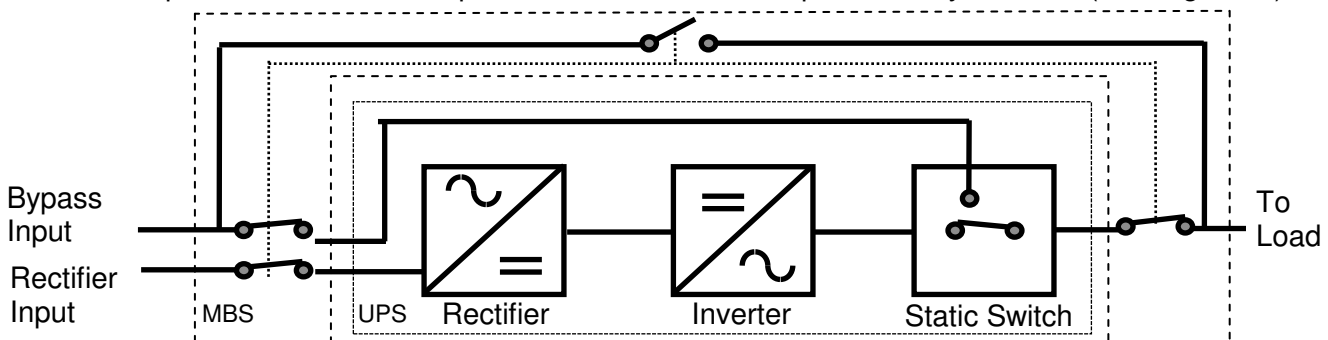
Figure 2. MBS in “Normal” Position
