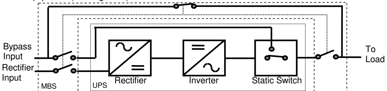
Figure 4. MBS in “Bypass” position
