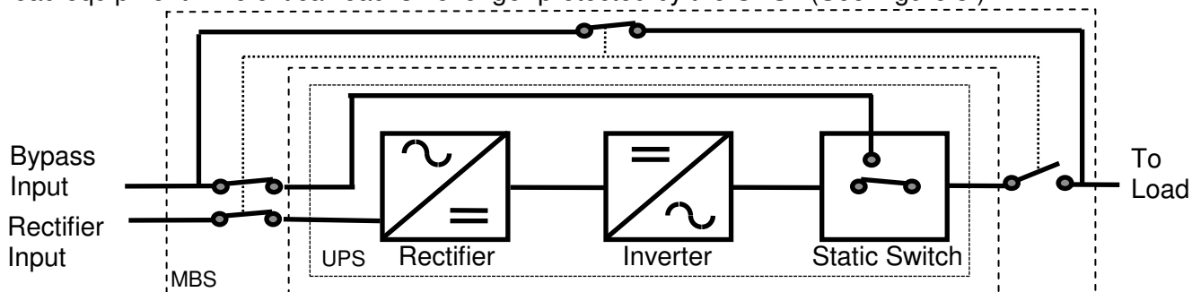
Figure 3. MBS in “Test” Position
