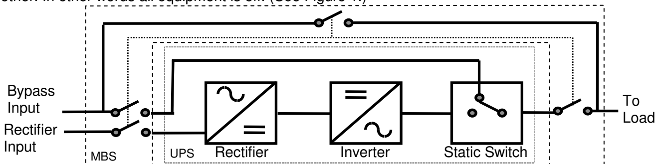
Figure 1. MBS in “Off” position
