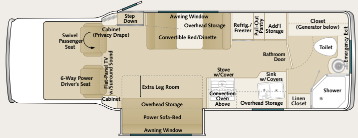
261XL SD Side Dinette with slideout
