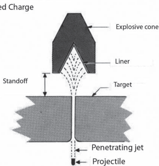
Figure 6. Shaped charge.
