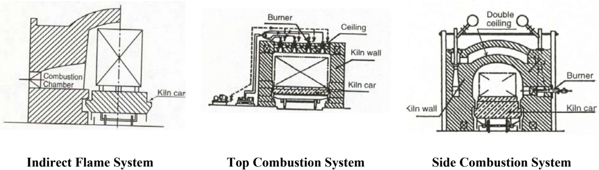
Figure 2-7. Tunnel Kiln
