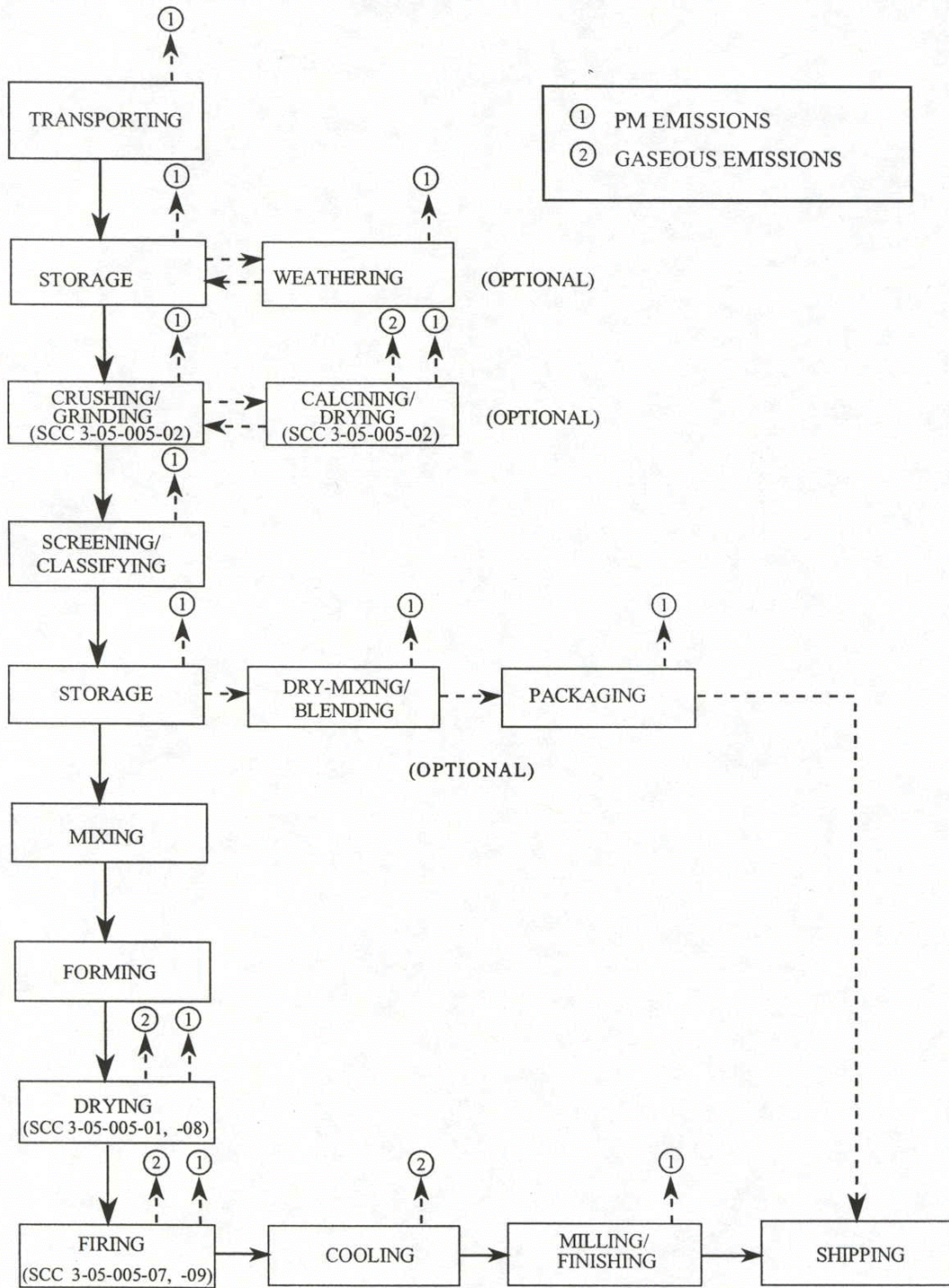
Figure 2-1a. Refractory Manufacturing Process Flow Diagram
