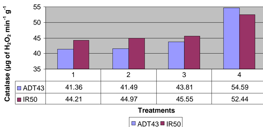
Figure 2. Effect of salt stress on catalase activity in two rice genotypes.
