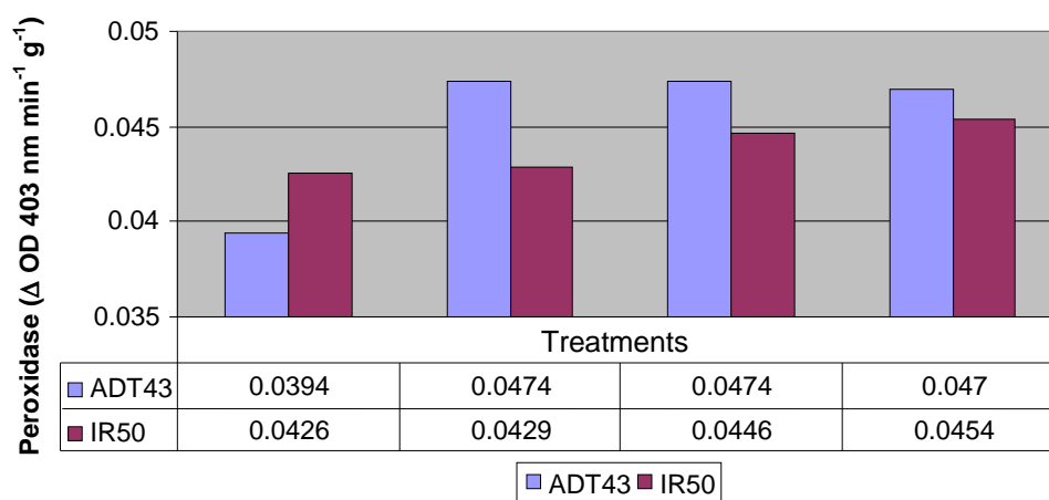
Figure 1. Effect of salt stress on peroxidase activity in two rice genotypes.
