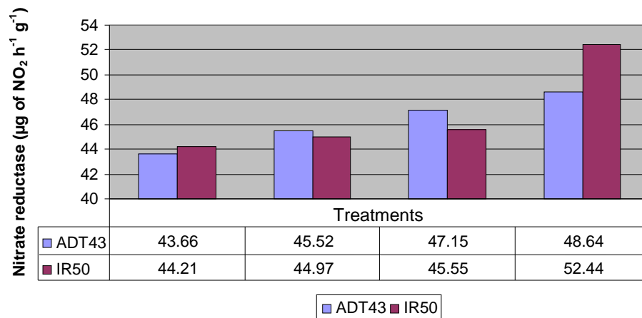
Figure 3. Effect of salt stress on nitrate reductase activity in two rice genotypes.
