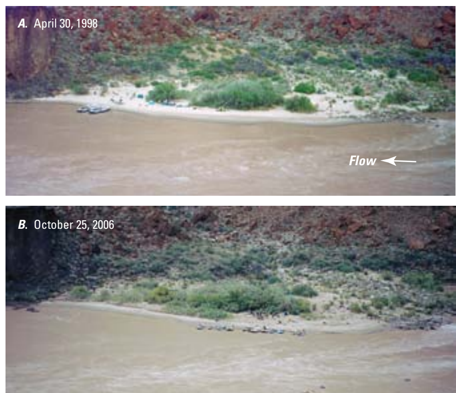
Figure 21. Repeat views looking across the Colorado River from the left bank at the sandbar and campsite located at river mile 202.3. Flow in main channel is from right to left. Between 1998 and 2006, woody vegetation, primarily arrowweed ( Pluchea sericea ), had expanded to cover large areas of the formerly sandy, unvegetated sandbar. A , Photograph taken April 30, 1998, at a river discharge of about 14,000 ft 3 /s. B , Photograph taken October 25, 2006, at a river discharge of about 11,700 ft 3 /s.
