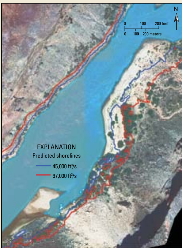
Virtual shorelines at Eminence Break camp (river mile 44). The blue shaded area (the river) shows the observed shoreline at a flow of 8,000 cubic feet per second (ft 3 /s) in the Colorado River at Lees Ferry, the blue line shows the predicted shoreline at 45,000 ft 3 /s, and the red line shows the predicted shoreline at 97,000 ft 3 /s. Modified from Magirl and others (2008).
