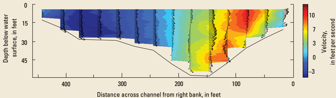
Cross-section view illustrating the three-dimensional characteristics of streamflow during the 2008 HFE. The view is looking downstream and shows the core of high-velocity flow far on the right side of the river. Filled contours are the downstream velocity component; downstream is red and upstream is blue. Arrows show vectors of cross-section and vertical-velocity components. Transect is located at the downstream end of the eddy depicted on the previous page (Wright and Kaplinski, in press).
