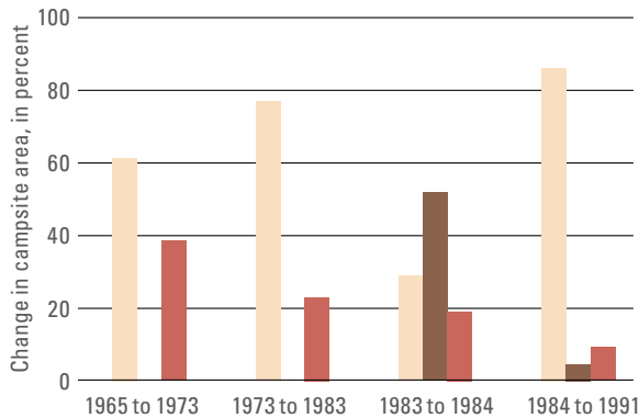
Figure 11. History of changes in campsites in Grand Canyon between 1965 and 1991 based on a composite of results from campsite inventories and aerial photograph interpretation. For each of four time intervals, the percentages of sites are shown that remained approximately the same size (tan), increased in size (brown), or decreased in size (red). Decreases in campsite size occurred in every time interval and the greatest decrease occurred between 1965 and 1973. Some campsites increased in size between 1983 and 1984 and between 1984 and 1991 in response to post-dam floods that occurred between the observations. Modified from Kearsley and others (1994).
