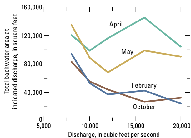
Figure 23. The relation between total backwater habitat area and discharge for the sandbar and backwater monitoring sites in 2008. Modified from Grams, Schmidt, and Andersen (2010).
