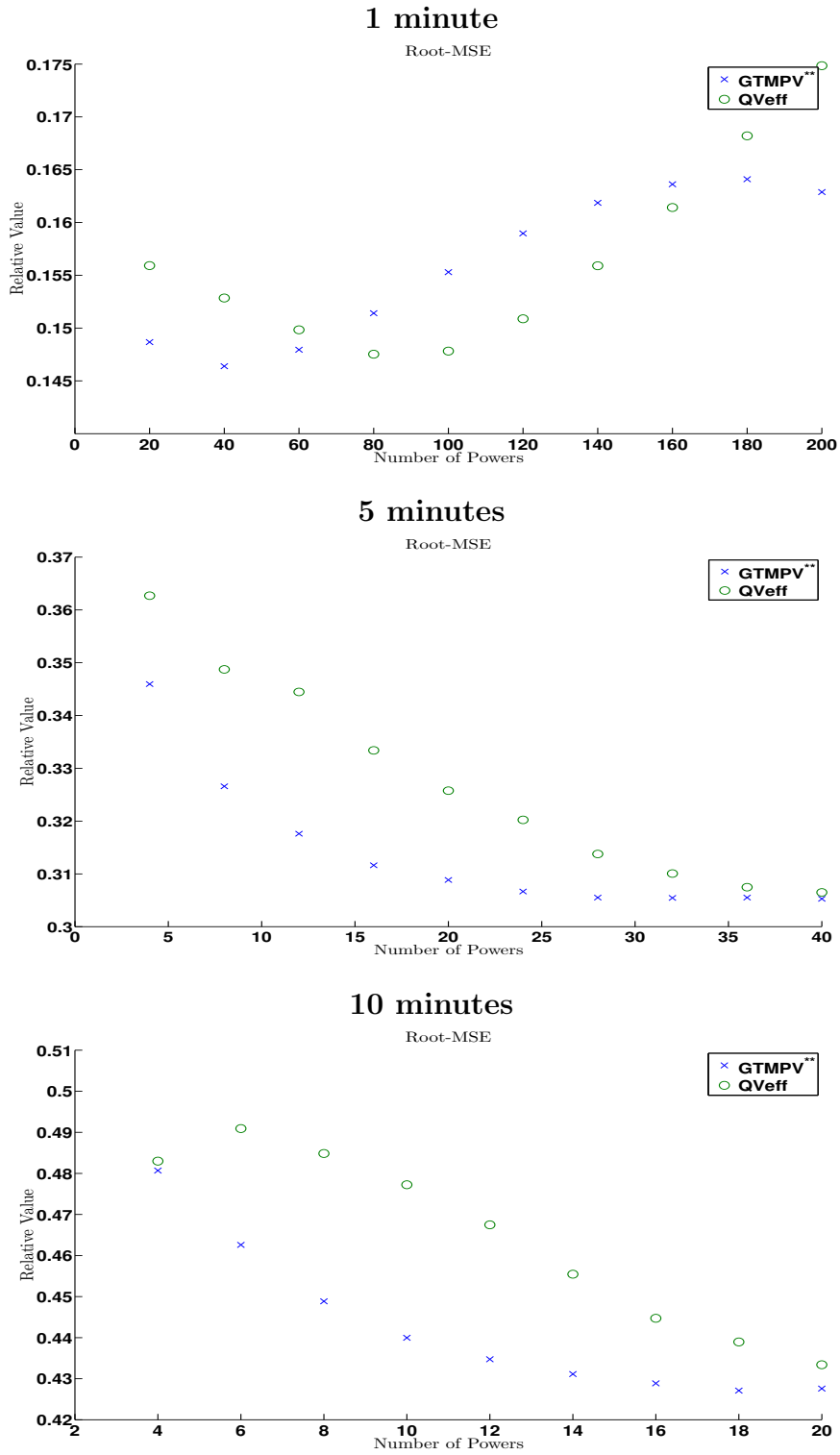
Figure 2: Relative RMSE obtained on simulations for the GTMPV^{**}(m) and QVeff , the Jacod and Rosenbaum estimator with k_n = m + 1 for different values of m , at three different sampling frequencies.
