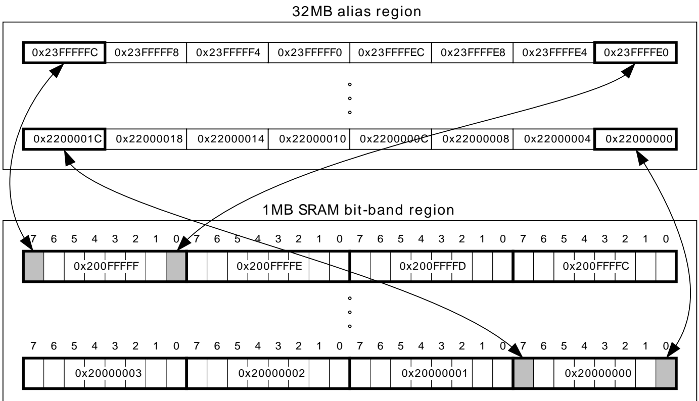
Figure 2.1. Bit-band mapping
