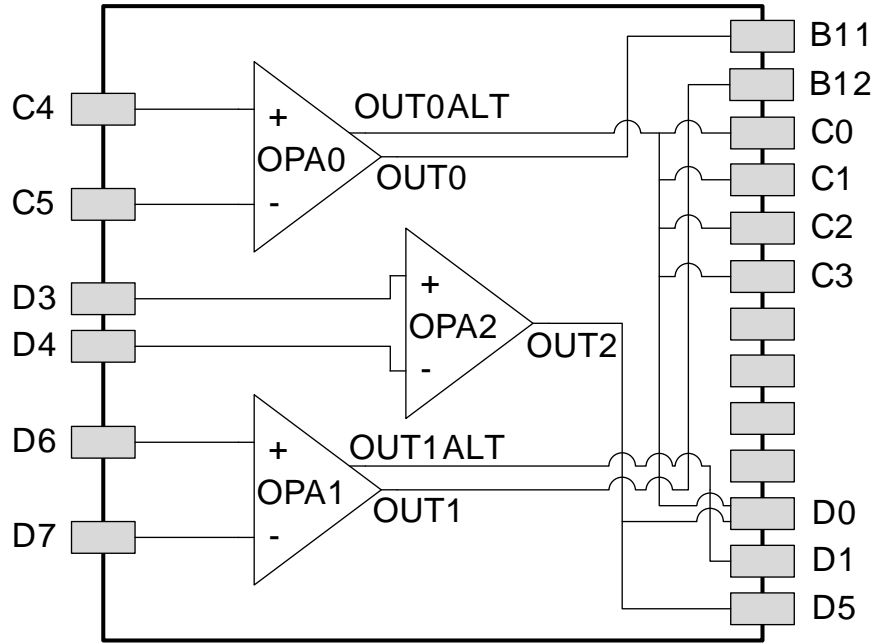
Figure 4.2. Opamp Pinout
