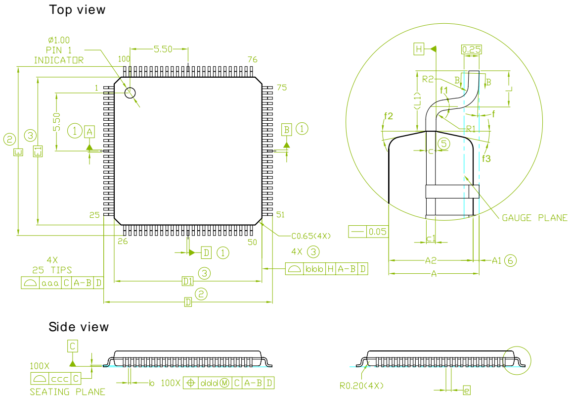
Figure 4.3. LQFP100
