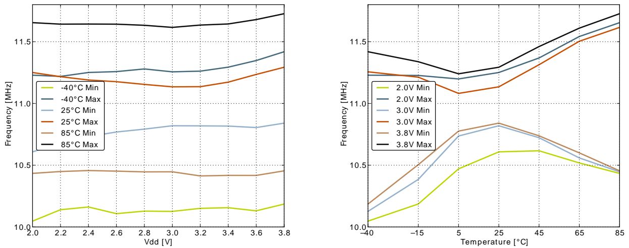
Figure 3.14. Calibrated HFRCO 14 MHz Band Frequency vs Supply Voltage and Temperature
