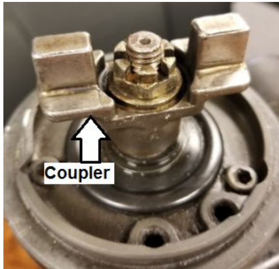
Figure 9: EA-19000 Coupler
