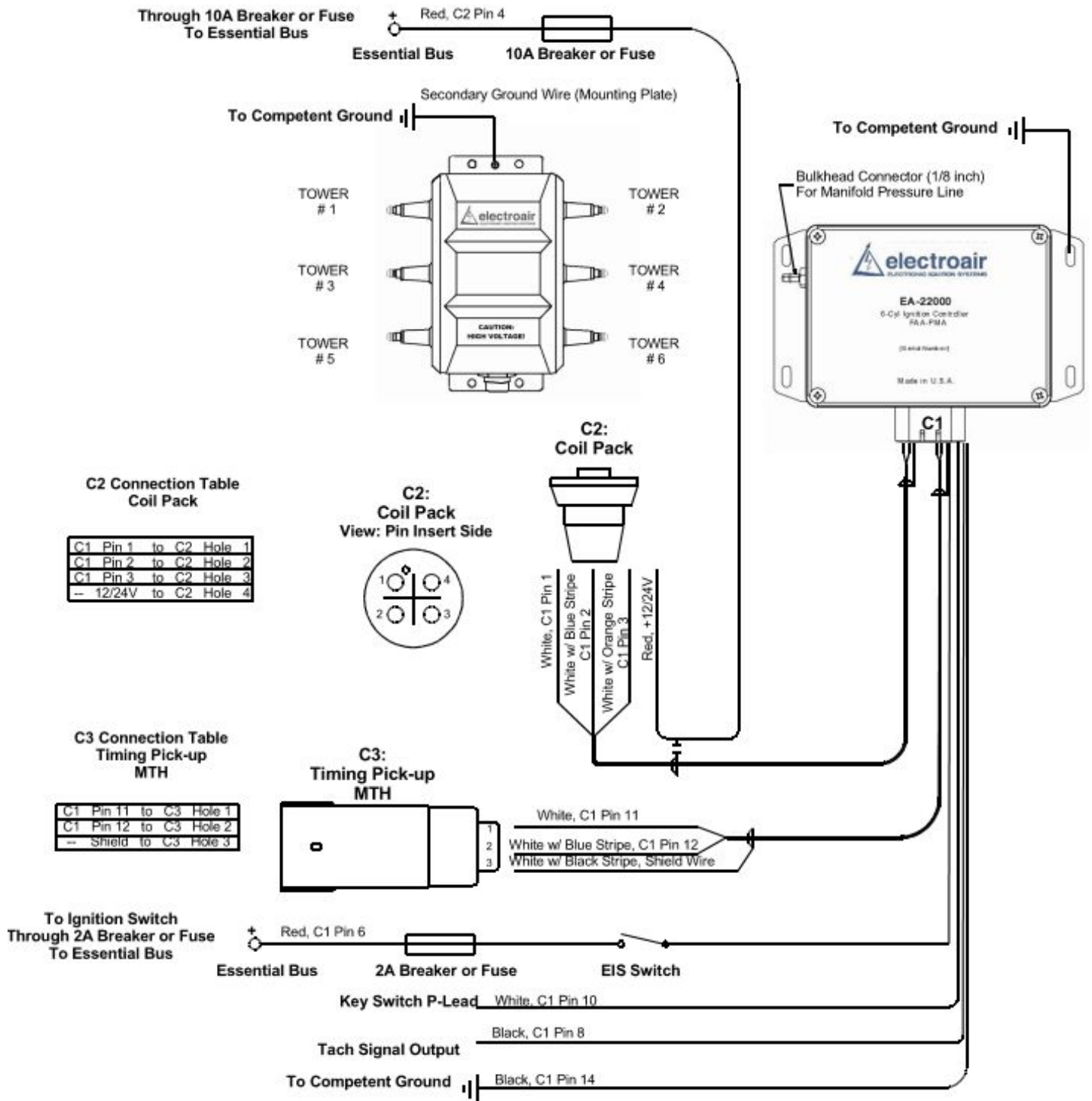
Figure 18: Wiring diagram for EIS-61000
