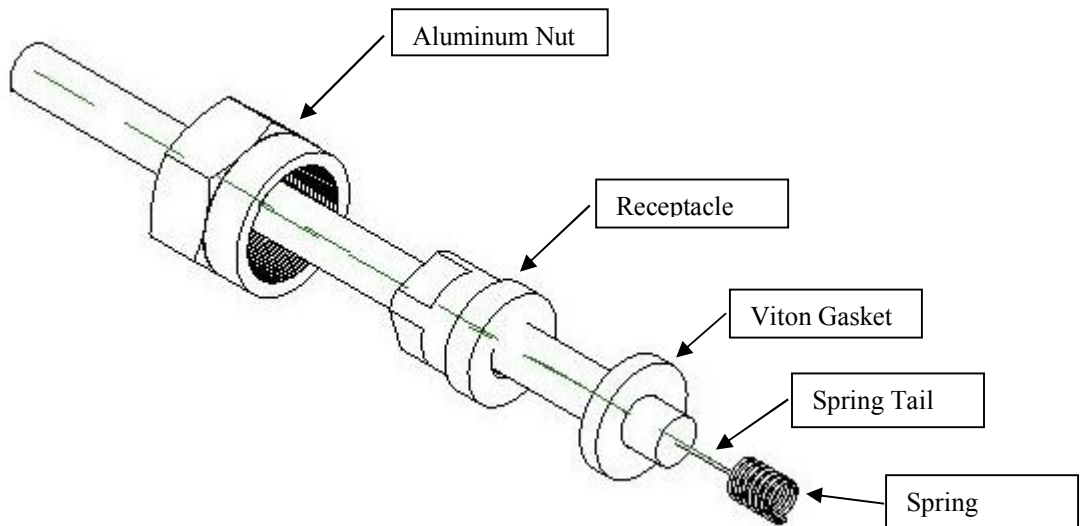
Figure 12: Spark Plug Wire Component Stack Up.
