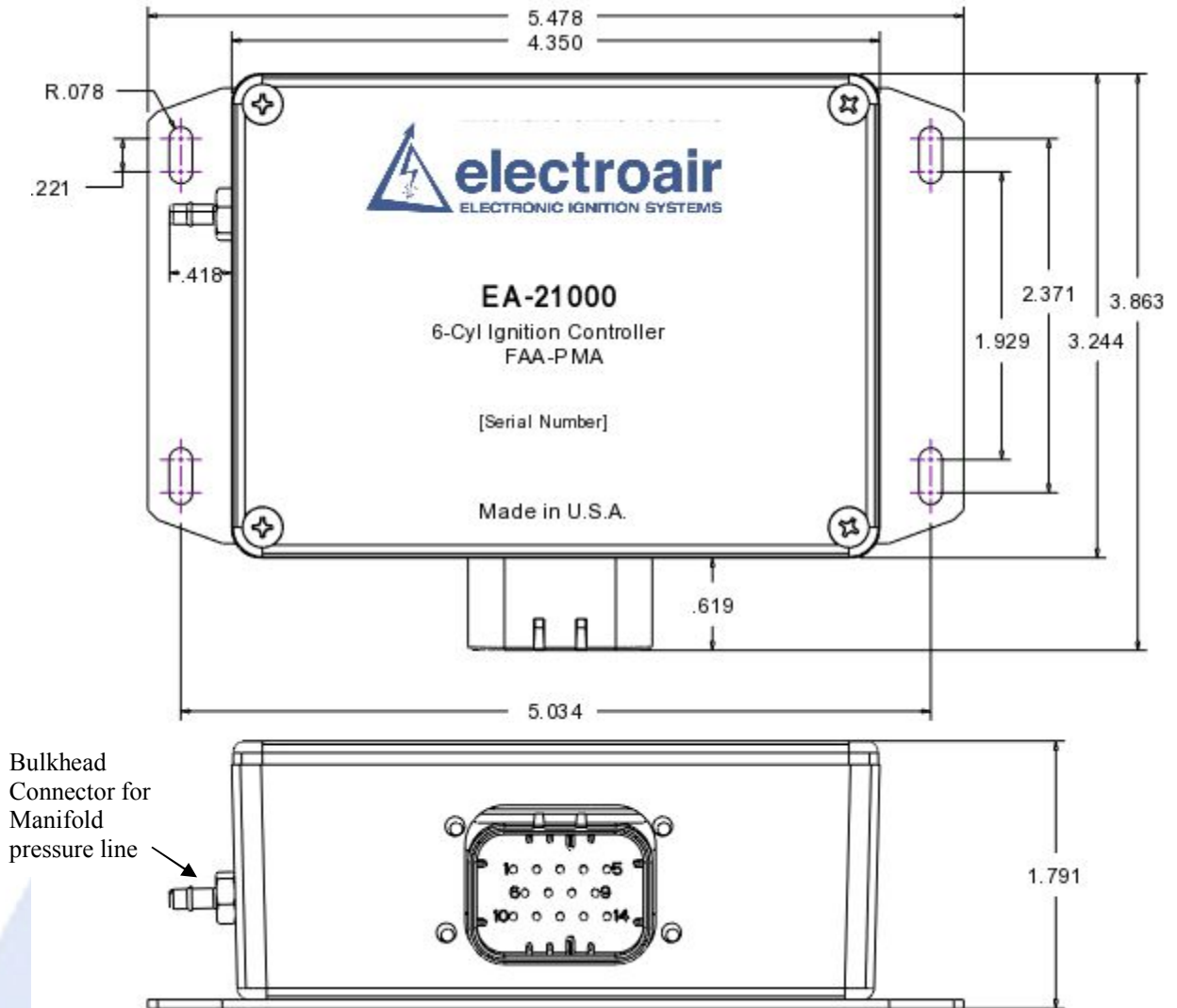
Figure 10: Part Number EA-21000; all dimensions in inches.
