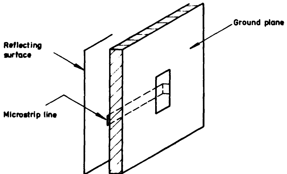
FIG. 2.9. THE GROUND PLANE SLOT RADIATOR
