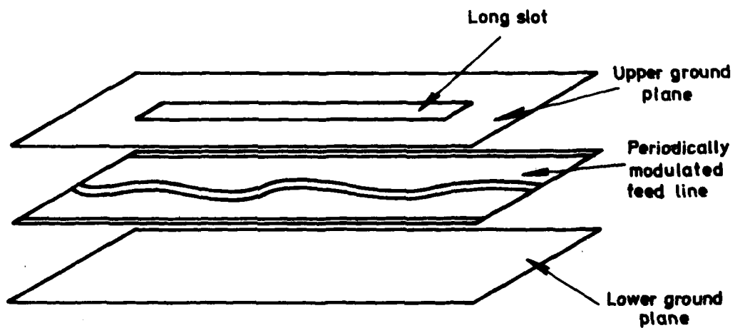
FIG. 3.6. PERIODICALLY MODULATED RADIATOR
