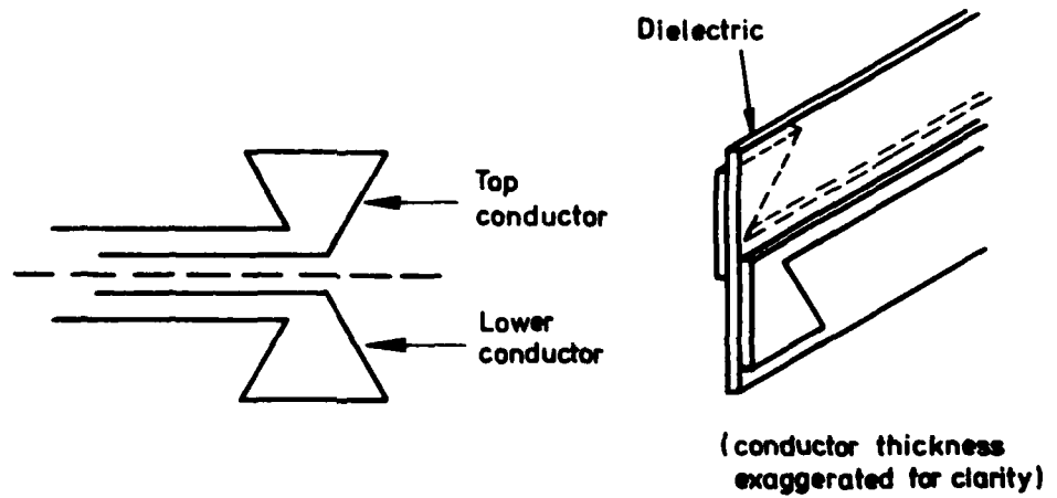
FIG. 2.4. PRINTED DIPOLE
