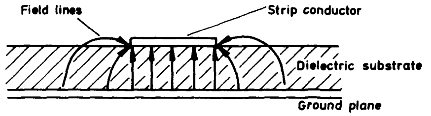
FIG 1. 1. MICROSTRIP TRANSMISSION LINE
