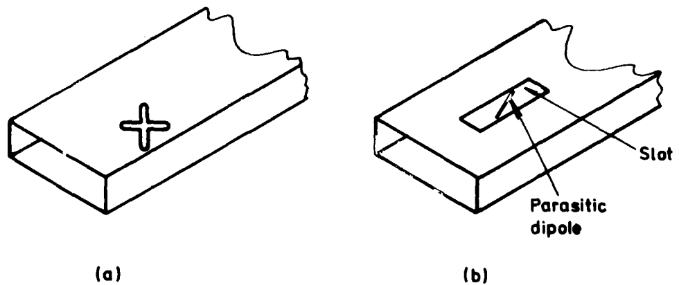
FIG. 4.9. CIRCULARLY POLARISED SLOT RADIATORS
