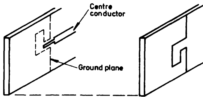
FIG. 2.5. STRIPLINE FED PRINTED DIPOLE
