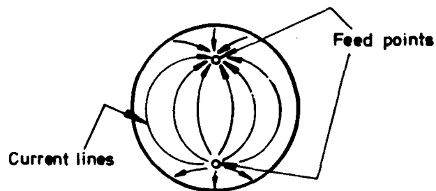
FIG. 1. 14. CIRCULAR RESONANT RADIATOR
