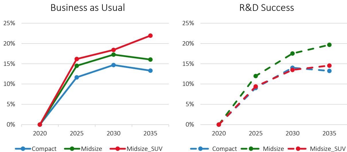
FIGURE 17: PROJECTED PERCENTAGE CHANGES IN MSRP OF CONVENTIONAL LIGHT-DUTY VEHICLES IN BAU TECH AND R&D SUCCESS SCENARIOS
