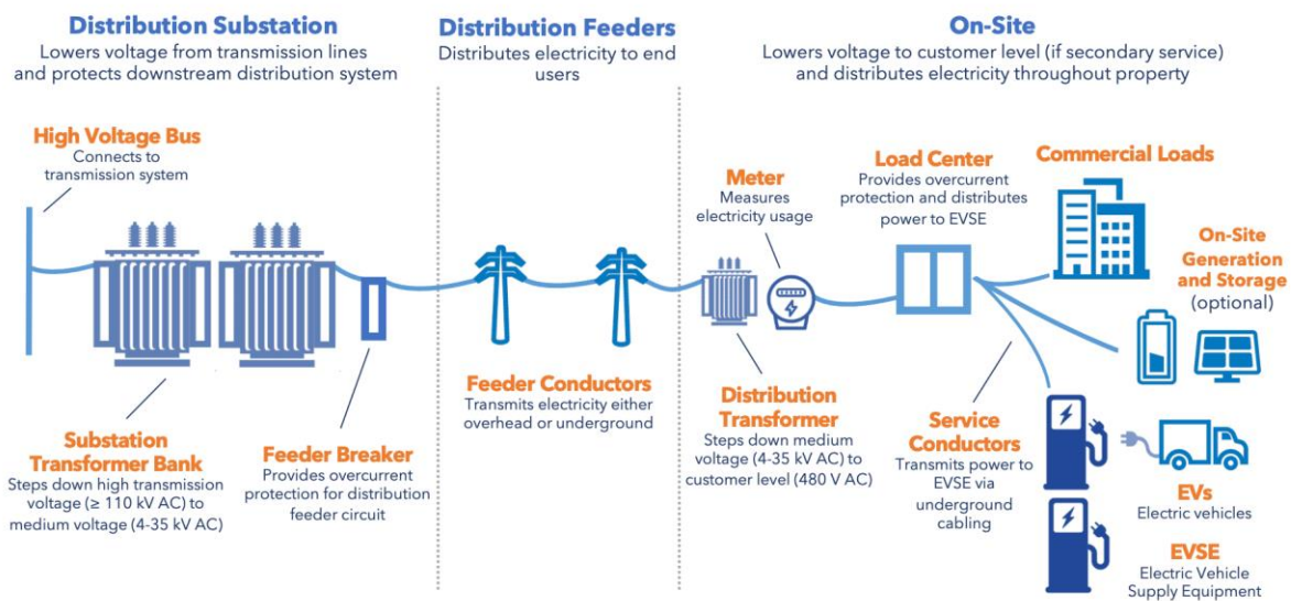
FIGURE 91: SCHEMATIC OF TYPICAL ELECTRICITY DISTRIBUTION COMPONENTS
