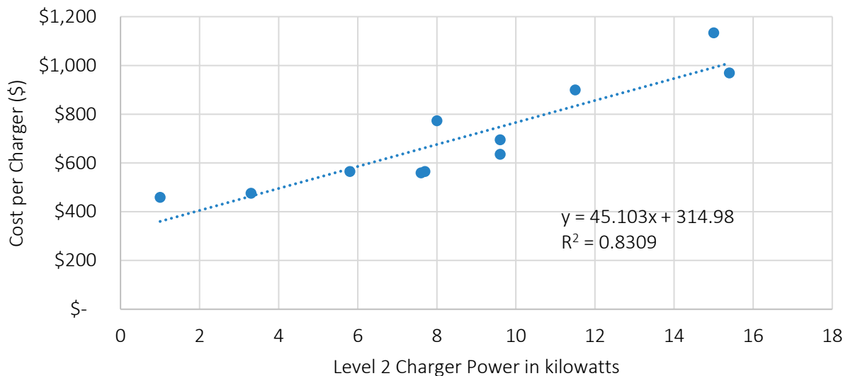
FIGURE 20: COST PER STATION AND POWER OF LEVEL 2 CHARGING STATIONS
