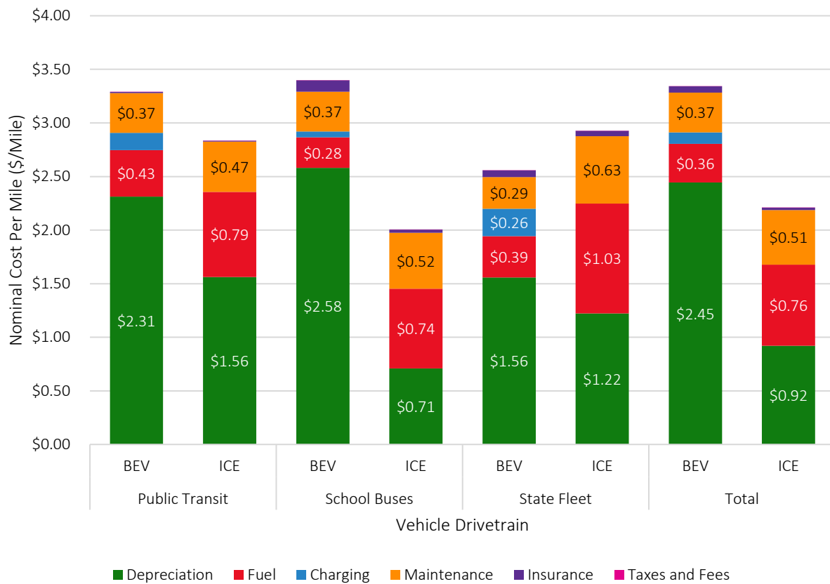
FIGURE 65: AVERAGE NOMINAL COST PER MILE BY DRIVETRAIN AND FLEET FOR HEAVY-DUTY VEHICLES
