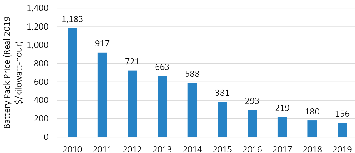
FIGURE 1: ESTIMATED BATTERY PACK PRICE (REAL 2019 $/KILOWATT-HOUR)
