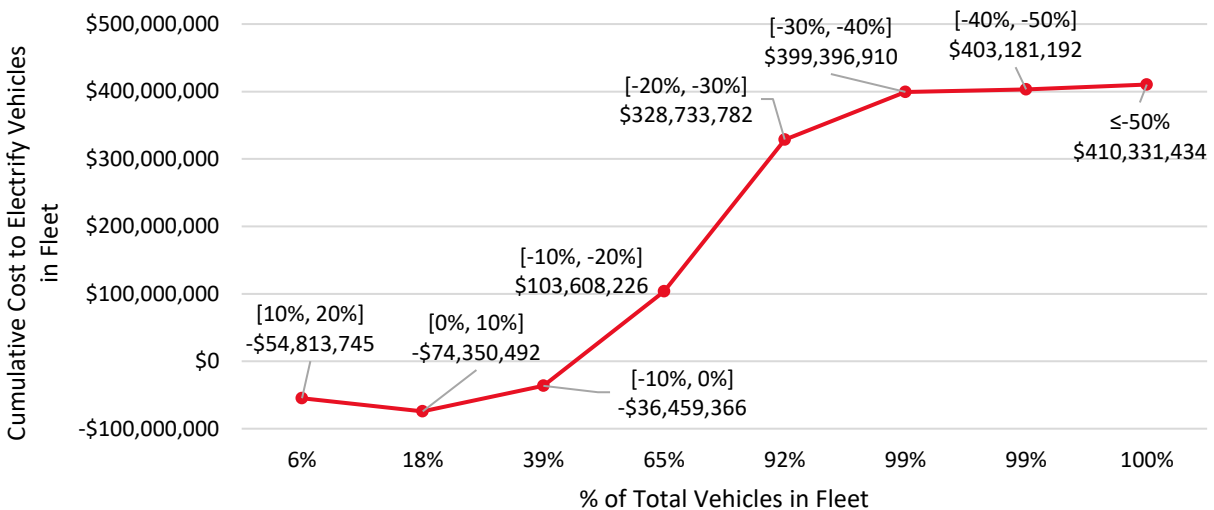
FIGURE 60: CUMULATIVE COST TO ELECTRIFY HEAVY-DUTY VEHICLES IN A SUBSEQUENT EV DEPLOYMENT
