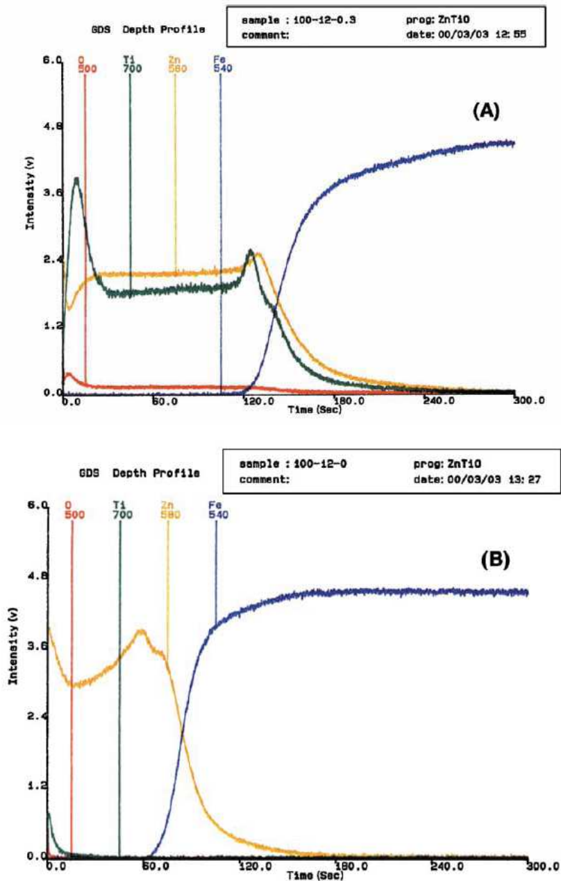
Fig. 8. GD-OES depth profiles for the TiO 2 -Zn nanocomposite films prepared at I_d = 12 \text{ A dm}^{-2} . A) TiO 2 -Zn(0.3,100)/Steel; B) TiO 2 -Zn(0,100)/Steel (Deguchi et al., 2001). (Reprint with the permission from Springer)
