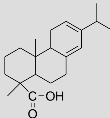
levopimaric acid
