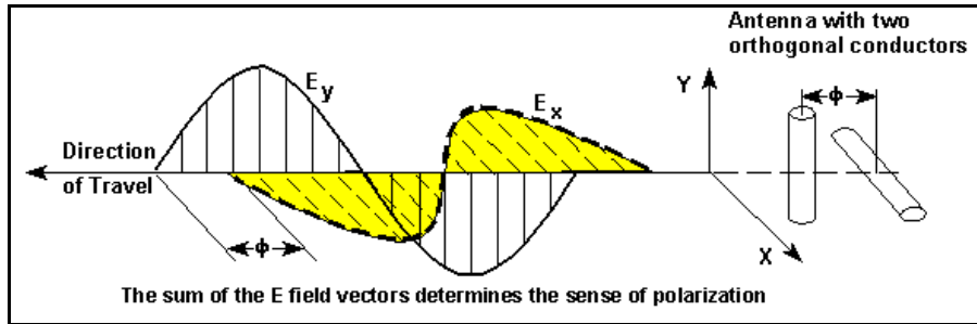
Figure1. Polarization Coordinates
