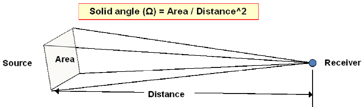
Figure 3. Solid Angle
