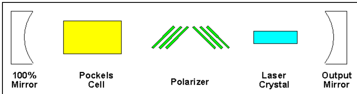
Figure 39. Q-Switch Arrangement
