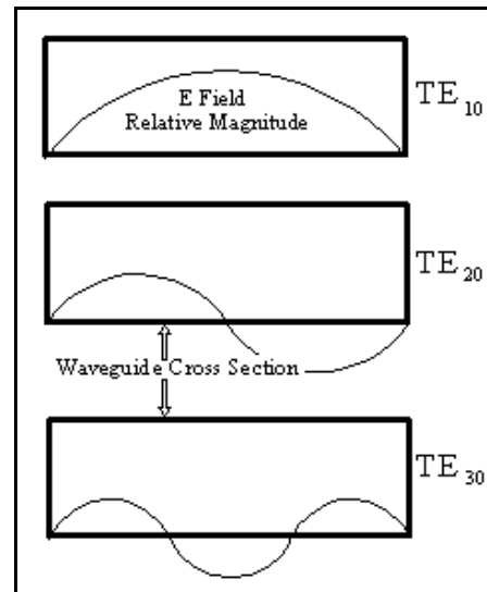
Figure 2. TE Modes
