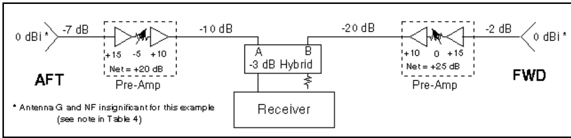
Figure 5. Example of Pre-Amplifier Affecting Overall Gain / Sensitivity
