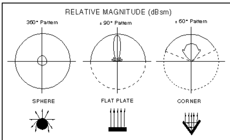
Figure 4. RCS Patterns
