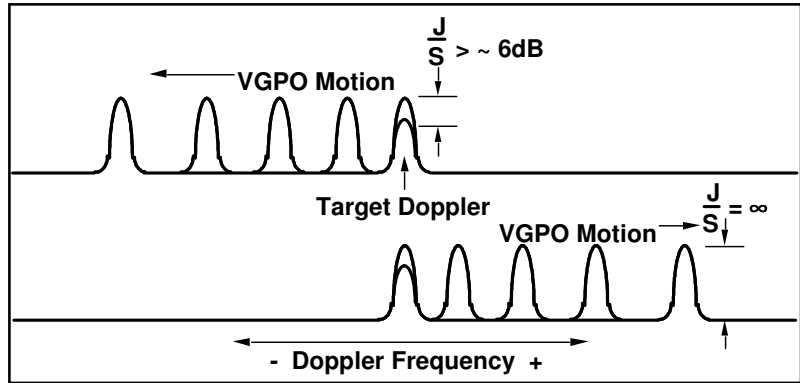
Figure 12. Velocity Gate Pull Off
