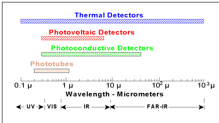
Figure 18. Spectral Range of Various Detectors
