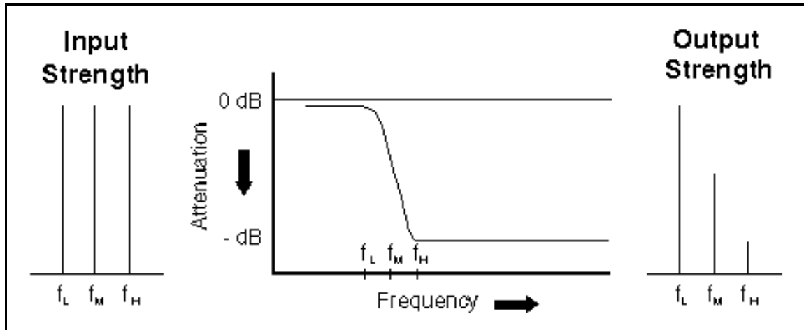
Figure 1. Low-Pass Filter
