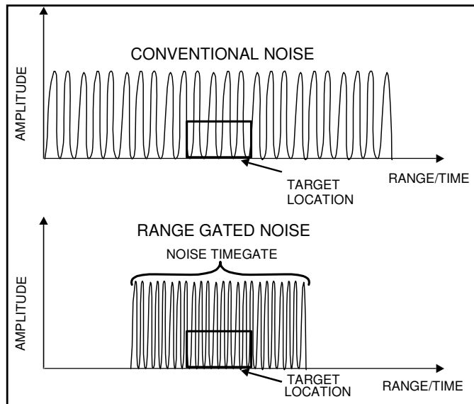
Figure 4. Noise Jamming
