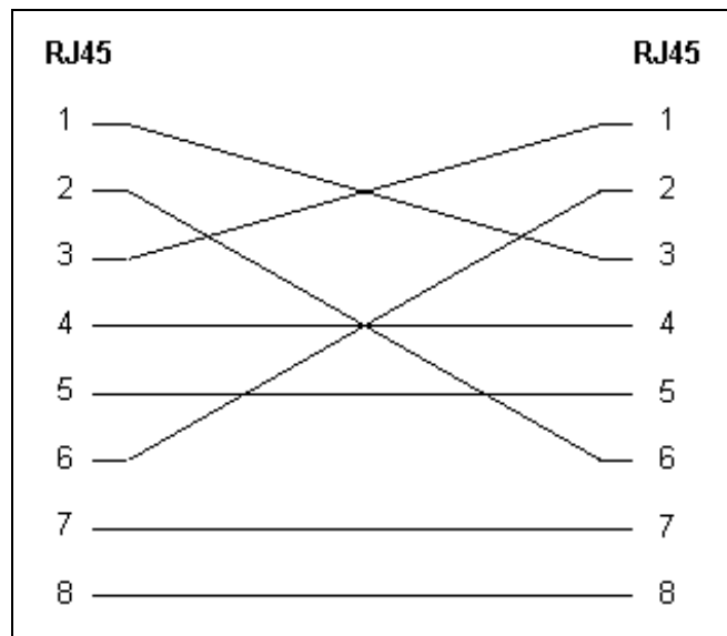
Figure 4. 10Base-T Crossover
