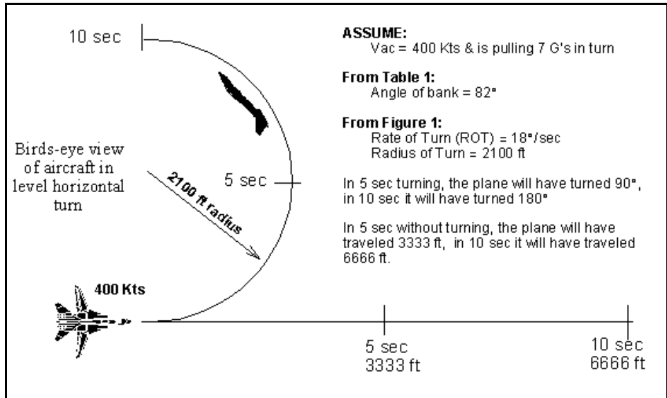
Figure 2. Maneuvering Aircraft
