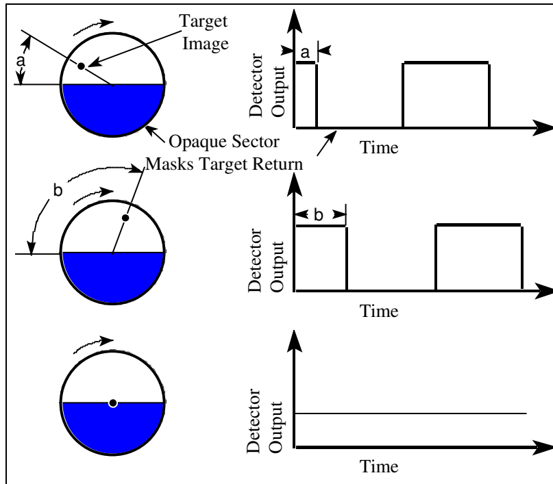
Figure 27. Basic Reticle Design
