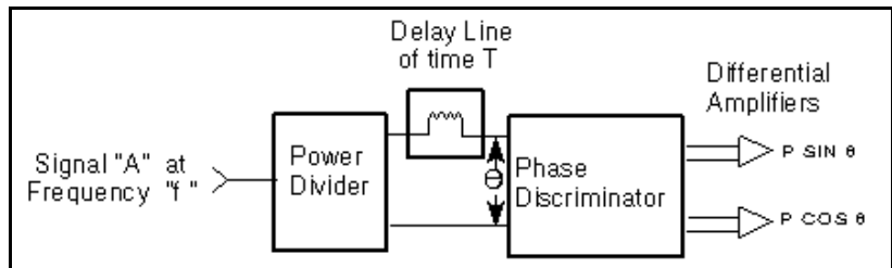
Figure 2. Frequency Discriminator
