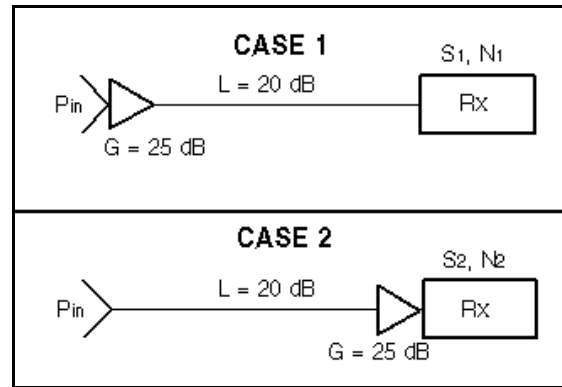
Figure 4. Pre-Amp S/N
