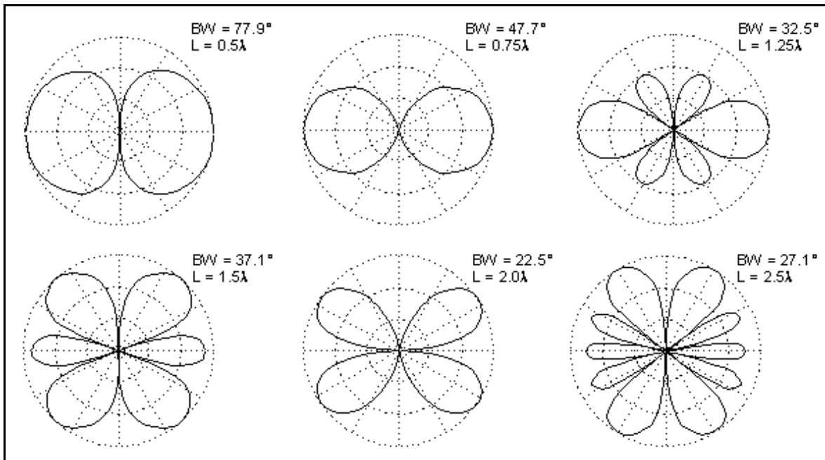
Figure 1. Frequency Effects
