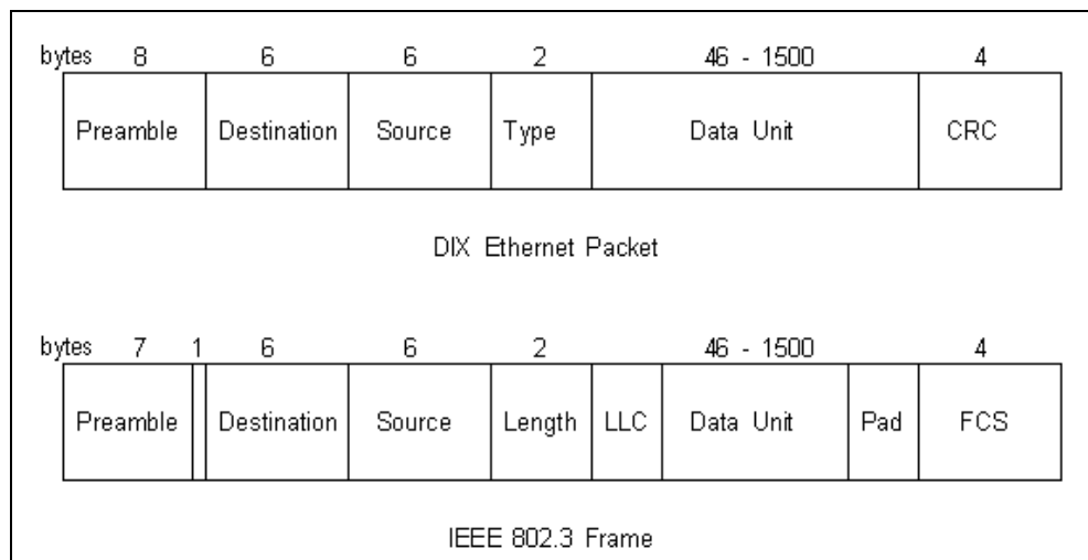
Figure 1. Ethernet Frame
