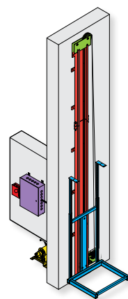
Custom Lift Winding Drum Series 210 Capacity 500 lbs
