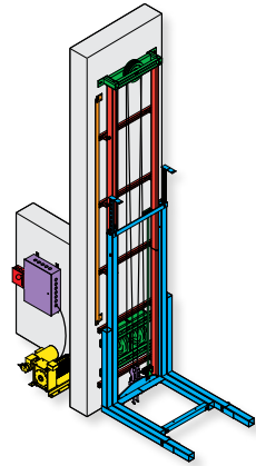
Paca-Lift, Winding Drum Series 118 / 018 Capacity 1,000 lbs
