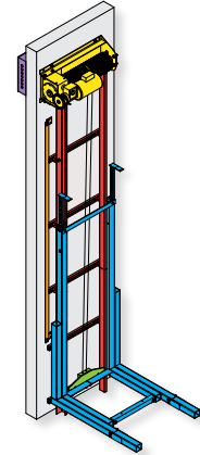
Paca-Glide, Winding Drum Machine Roomless Series 115 / 015 Capacity 1,000 lbs
