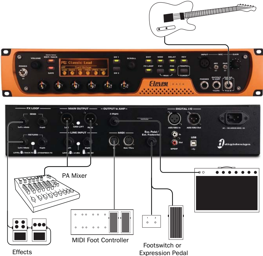
Figure 4. Eleven Rack Live Setup
