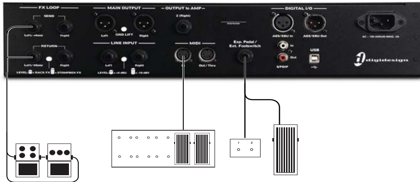
Figure 7. Effects and foot controller connections
