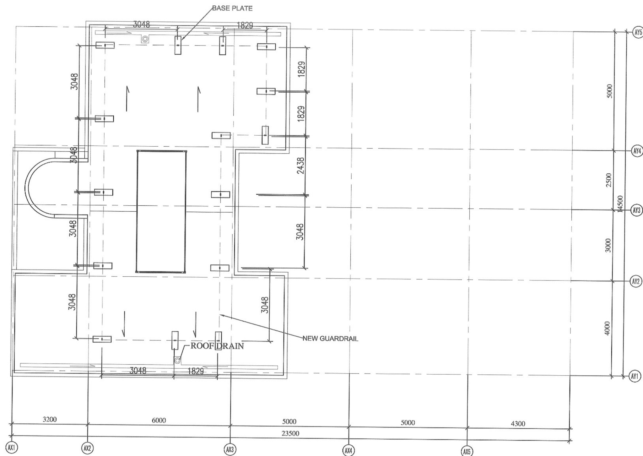
BUILDING "R1&R2" ROOF PLAN
