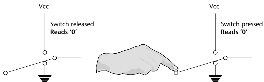
FIGURE 4.6 A schematic representation of a switch connected to a port ( without internal pull-up resistors). See text for details
