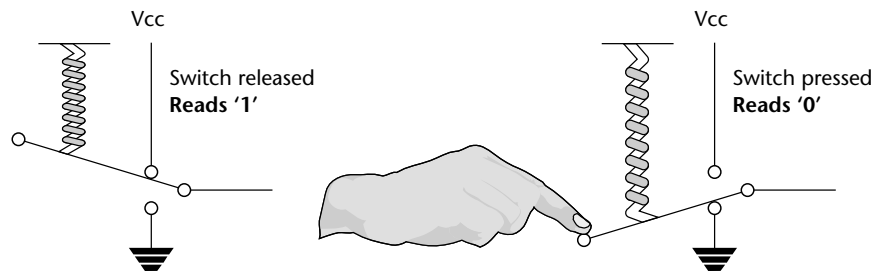
FIGURE 4.5 A schematic representation of a switch connected to a port (with internal pull-up resistors). See text for details
