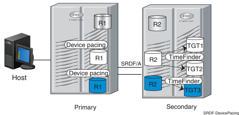
Figure 28 SRDF/A device pacing activated for R1 volumes
