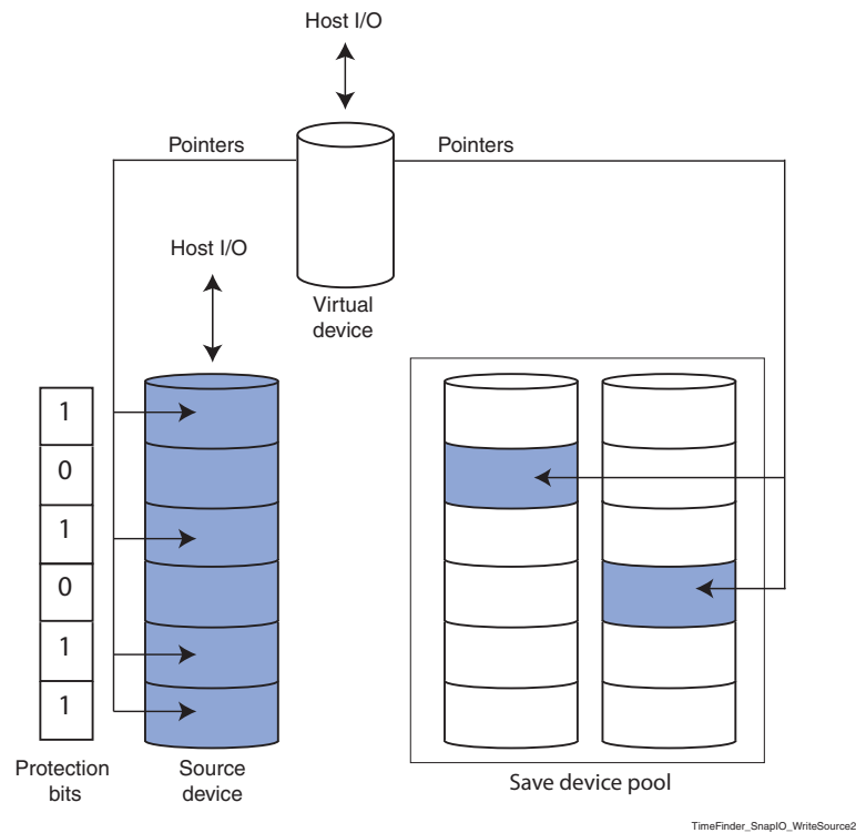
Figure 21 Pointers after data has been copied to the SAVE devices
