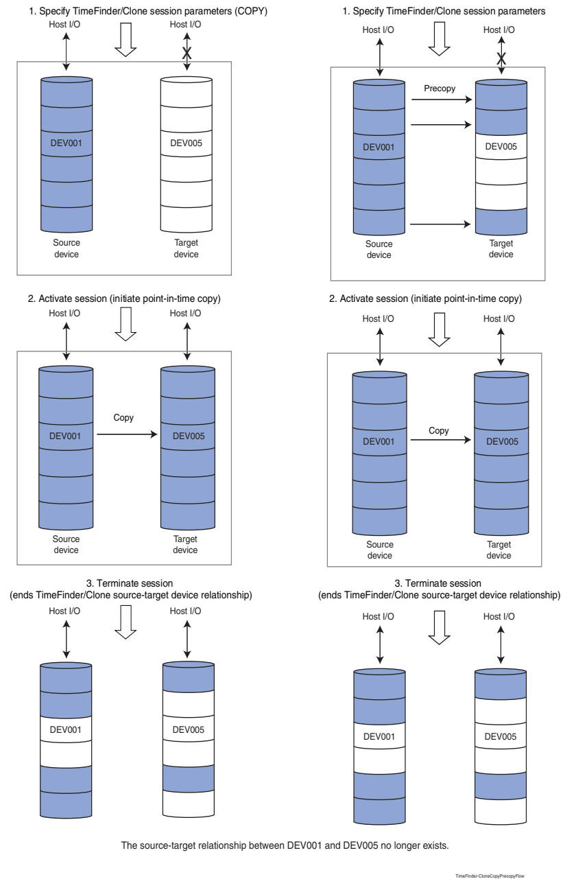
Figure 12 Full device clone sessions using copy and copy with precopy
