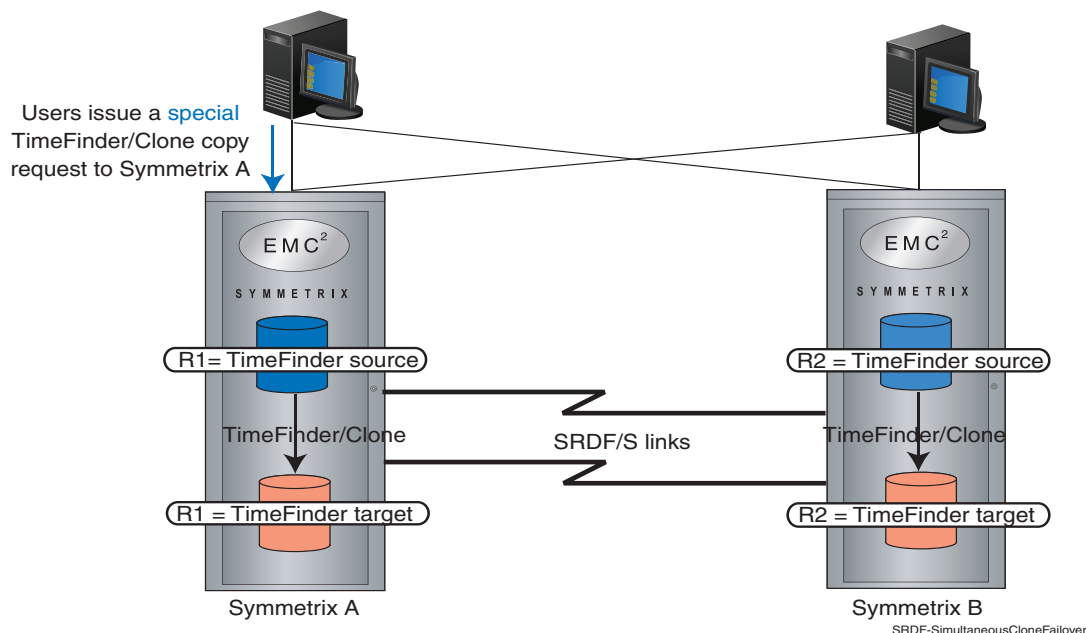
Figure 27 Simultaneous TimeFinder/Clone with Enginuity version 5875
