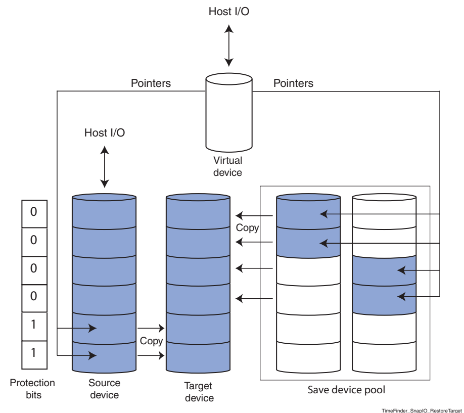
Figure 24 Fully restoring to a target device
