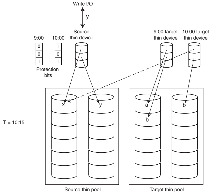
Figure 18 TimeFinder/Clone with Virtual Provisioning: 10:00 session after host write I/O
