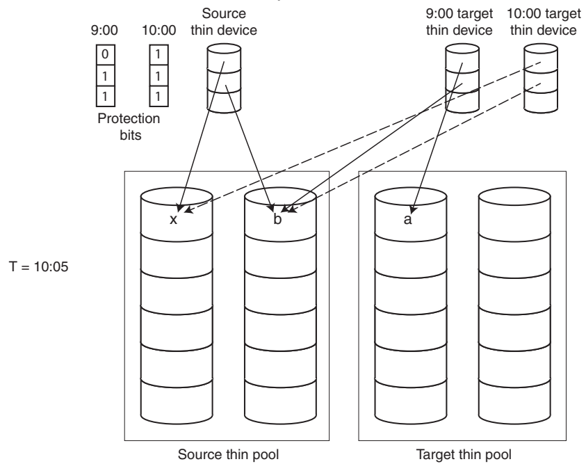
Figure 17 TimeFinder/Clone with Virtual Provisioning: 10:00 session before host write I/O
