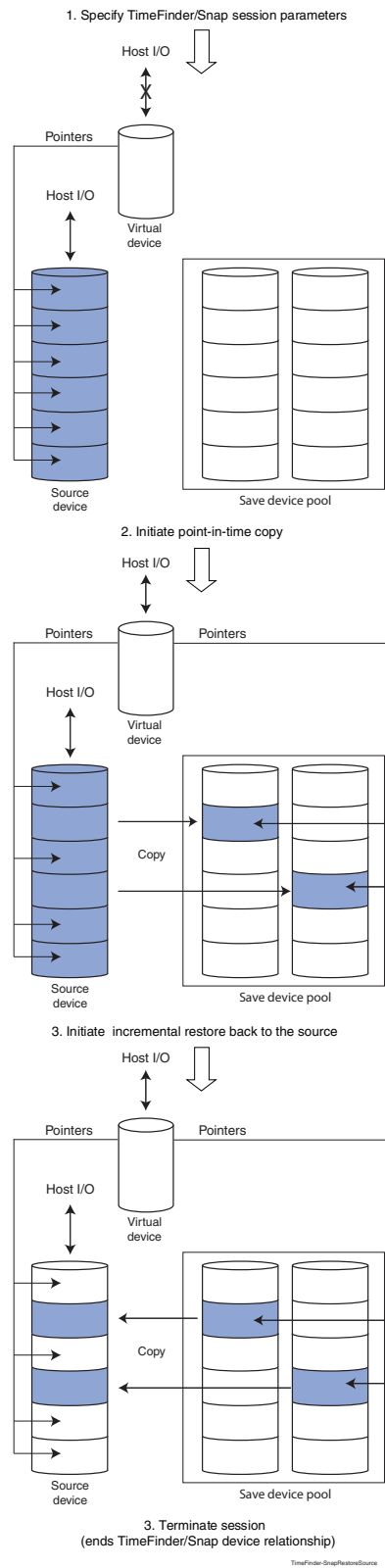
Figure 23 Incrementally restoring back to the source device
