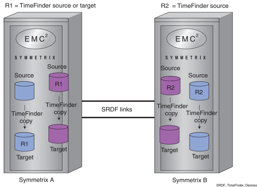
Figure 26 R1 devices as source and target devices in TimeFinder operations.
