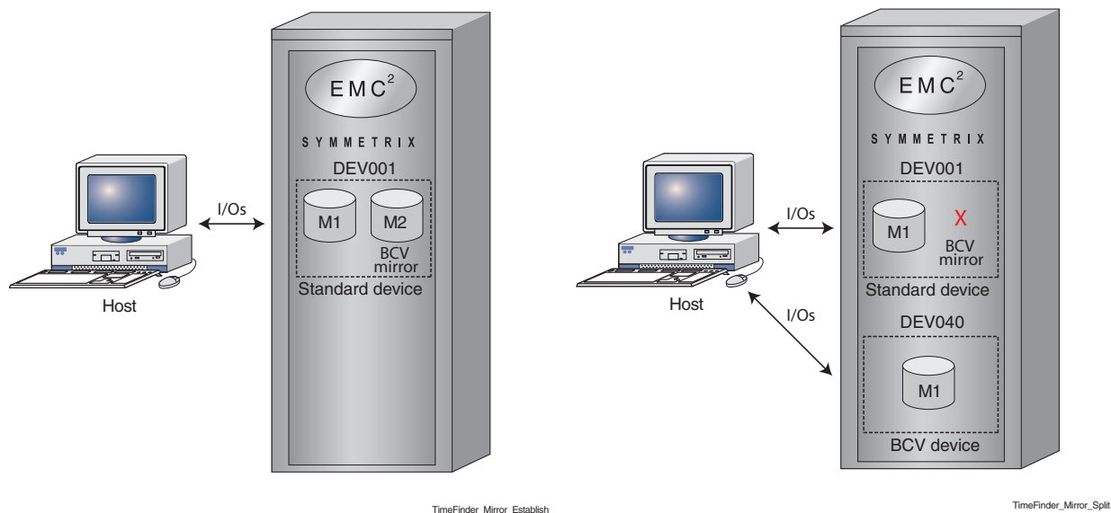
Figure 31 Standard device with an established BCV mirror
