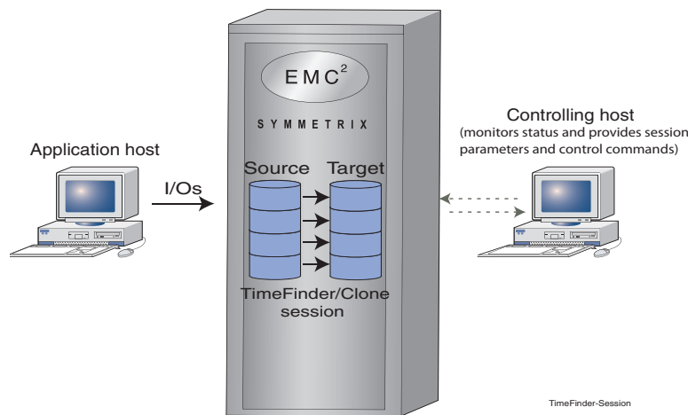
Figure 9 TimeFinder/Clone session
