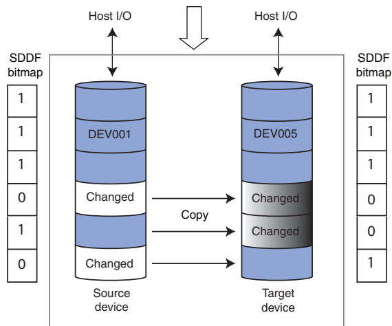
Figure 14 Full device clone session followed by an incremental clone copy
