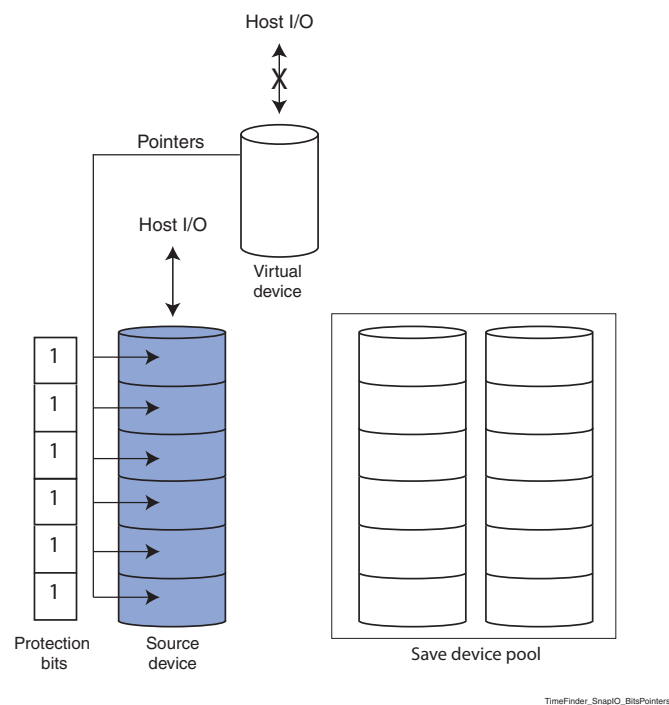
Figure 19 Protection bits and pointers
