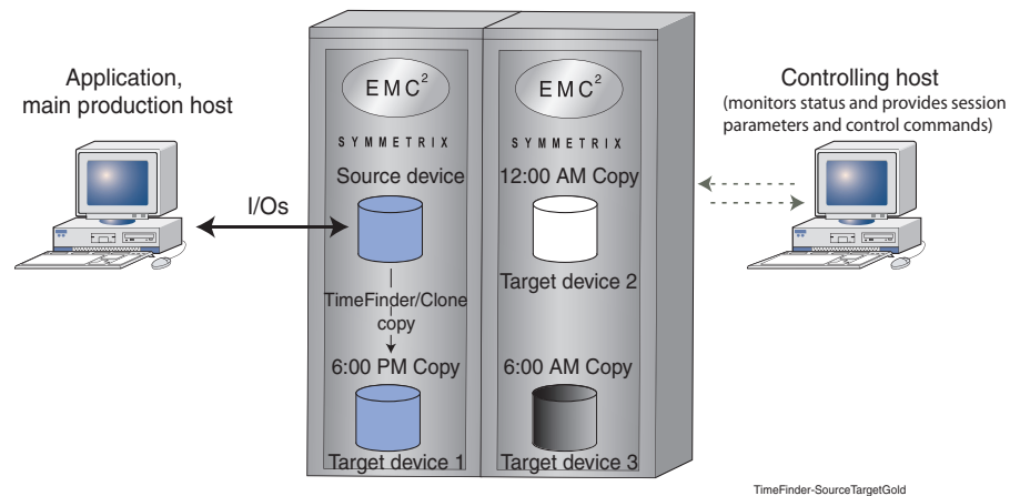
Figure 5 Target device keeping point-in-time copies
