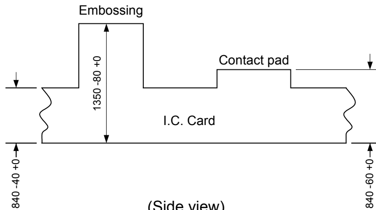
(Side view) Dimensions in \mu\text{m}
