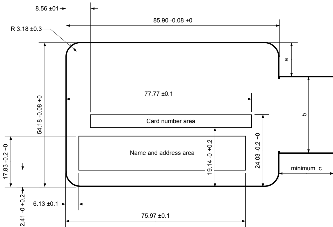
(Top view) Dimensions in mm
