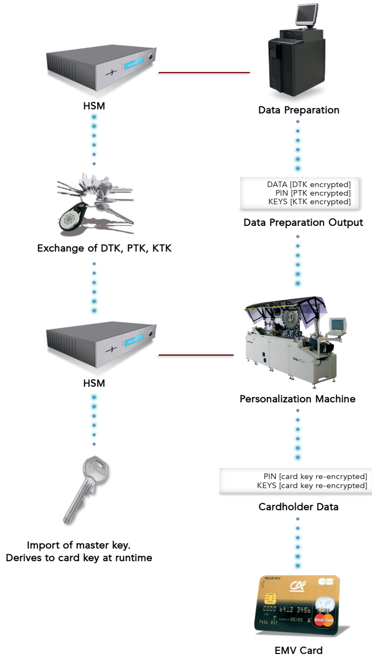
Figure 7: Personalization Cryptography
