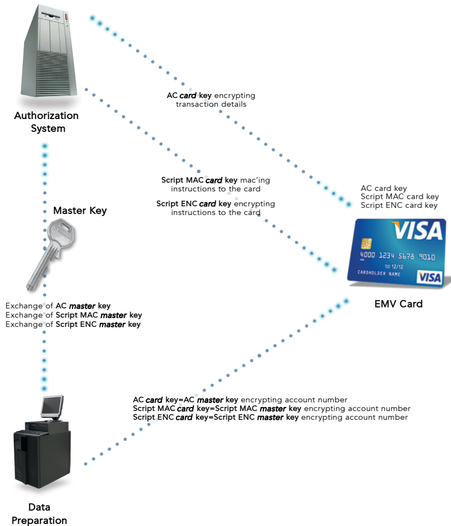
Figure 3: Sharing Keys
