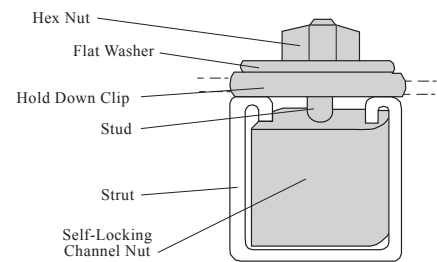
Diagram: FRP/GRP Channel Nut with Hold Down Clip
