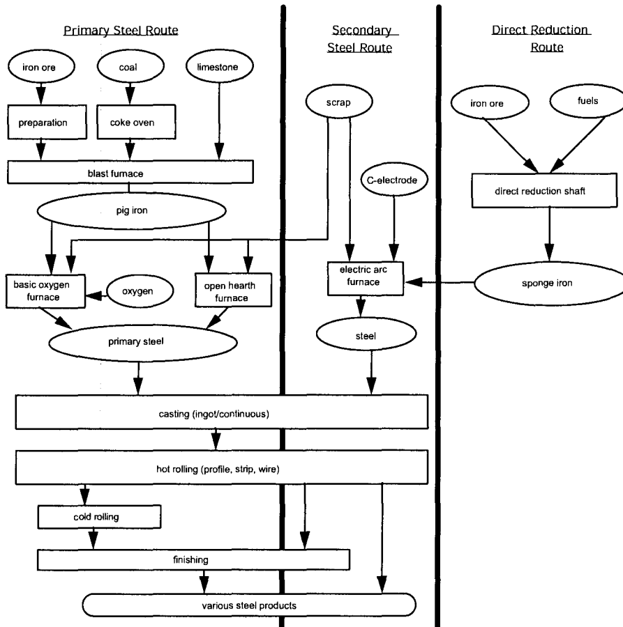
Figure A-1. Iron and Steel Production Routes
