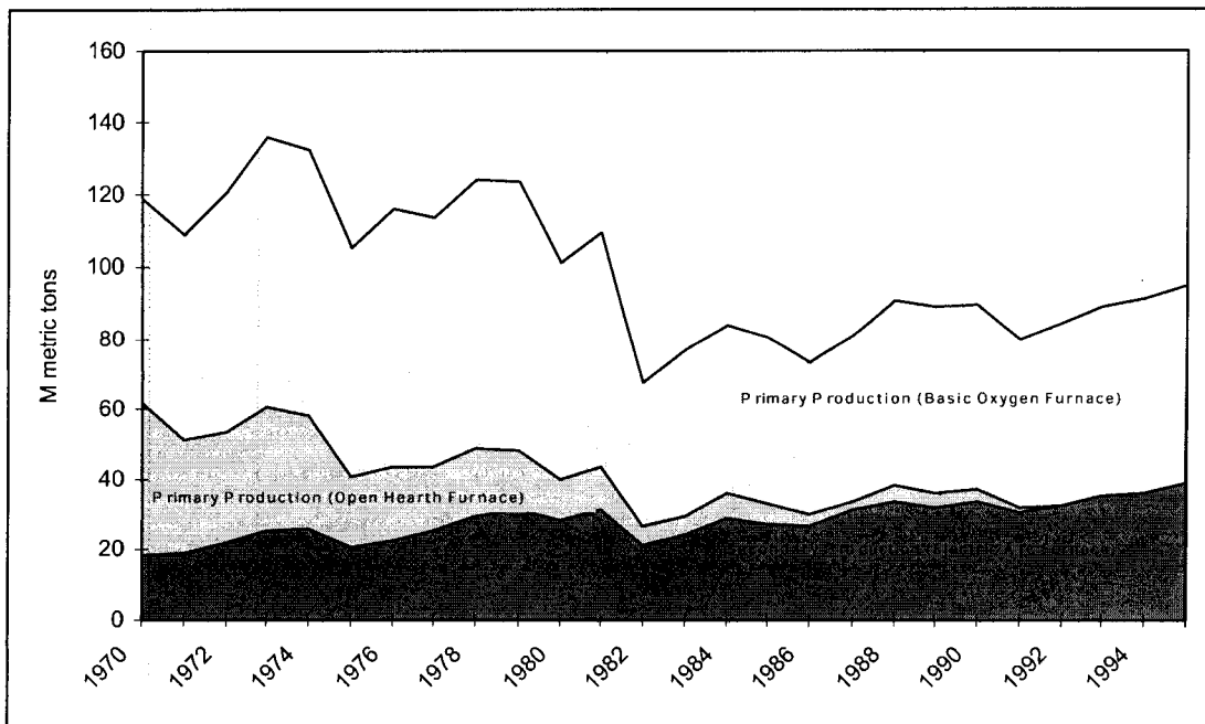
Figure 2. U.S. Steel Production by Process, 1970 to 1995.
